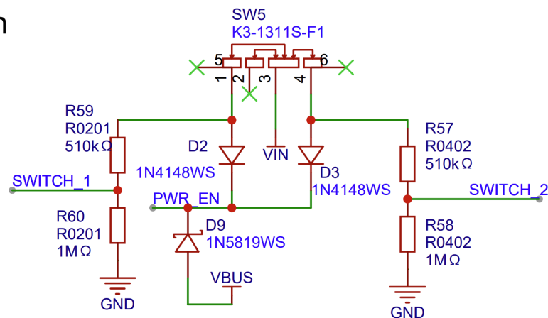
Fig. 3: Mode Switch Circuit Diagram (Click to enlarge)
