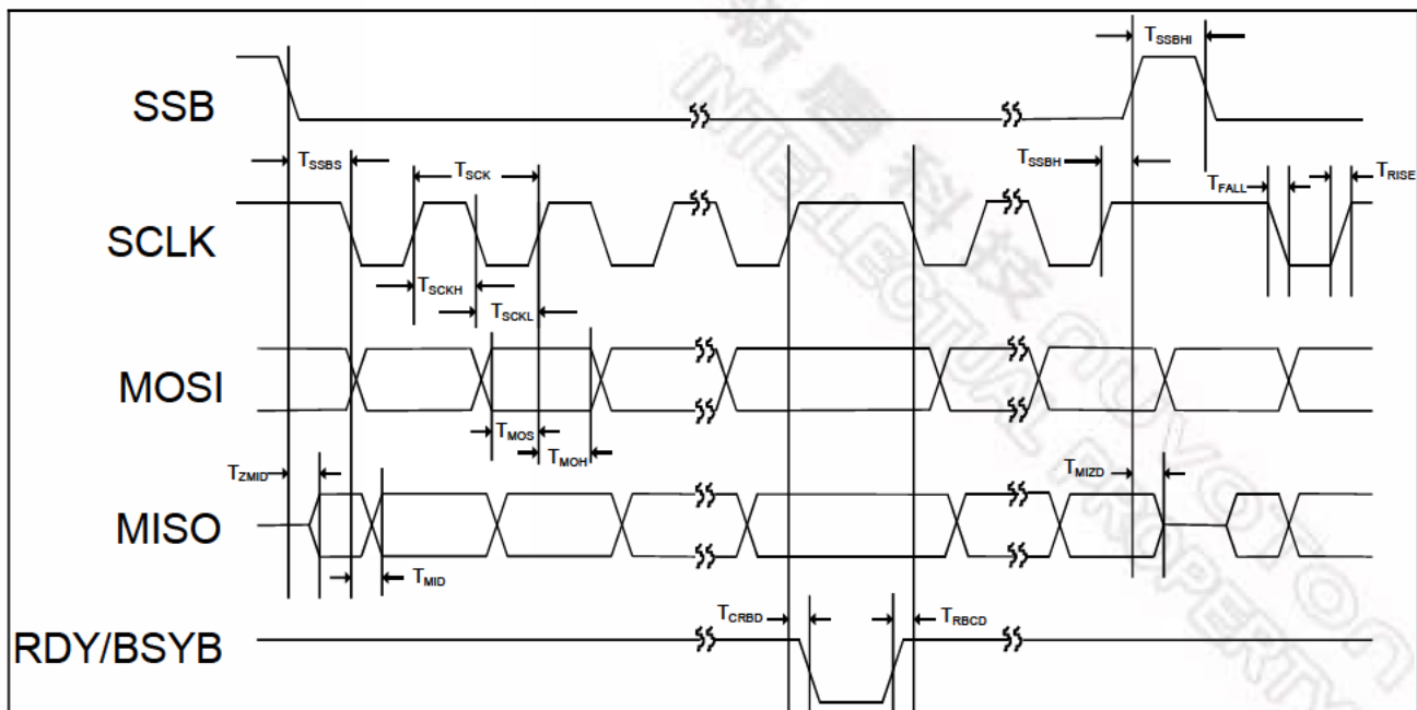
Figure 11-1 SPI Timing
