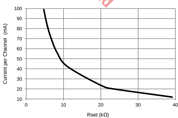
Fig. 9: Current per Channel vs RSET resistor
