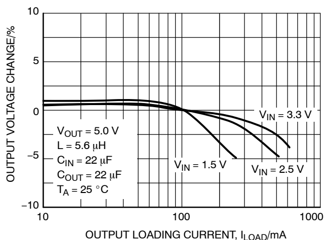
Figure 15. Output Voltage Change vs. Load Current
