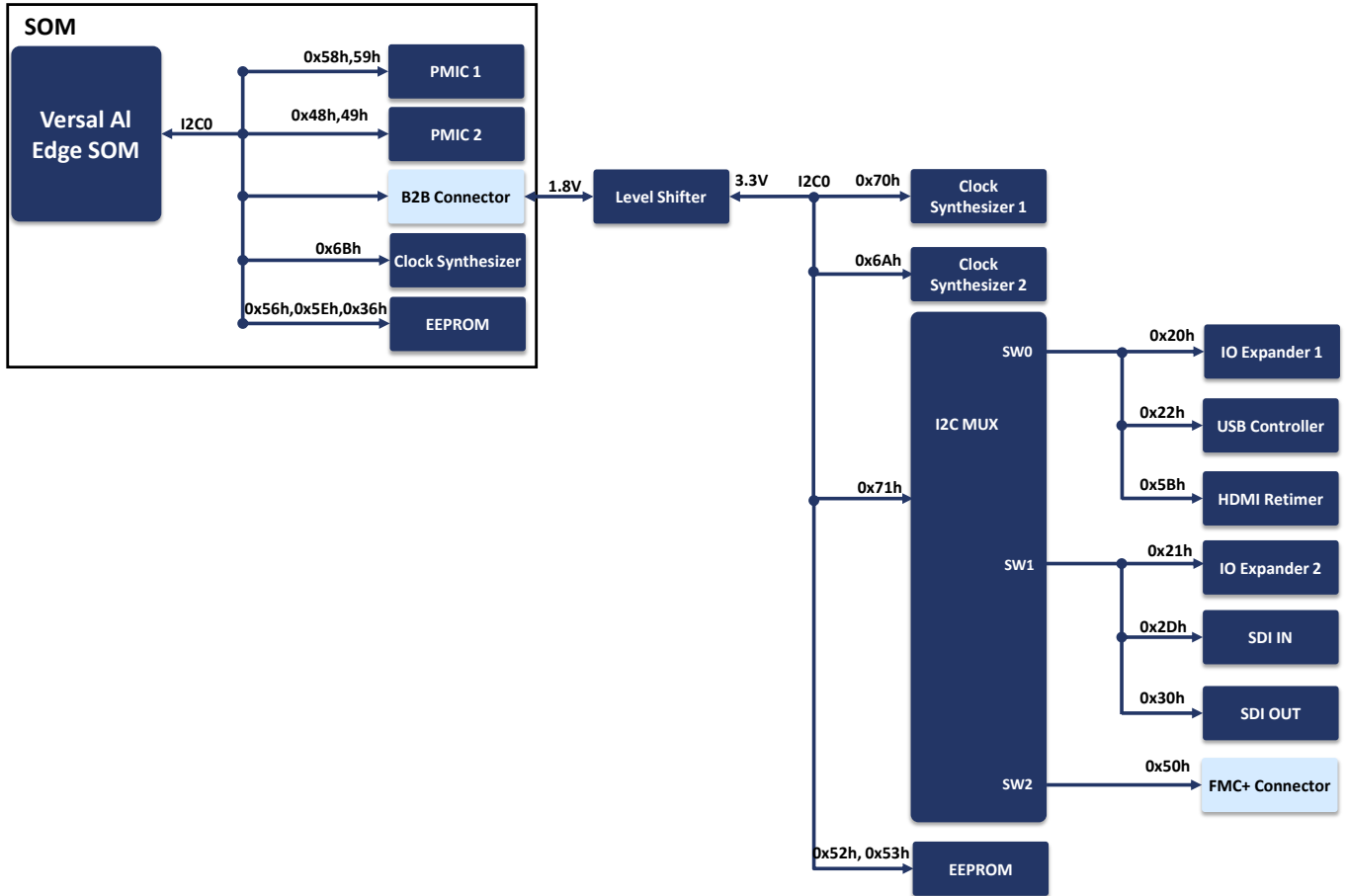
Figure 19: I2C Tree
