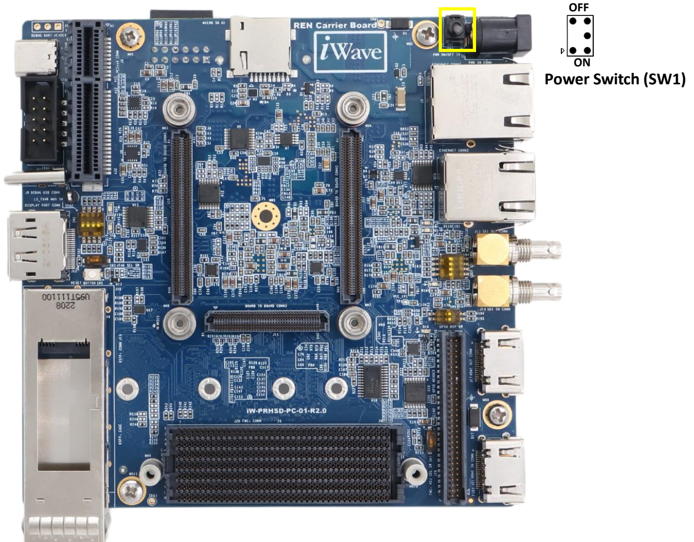
Figure 20: Power On/Off Switch
