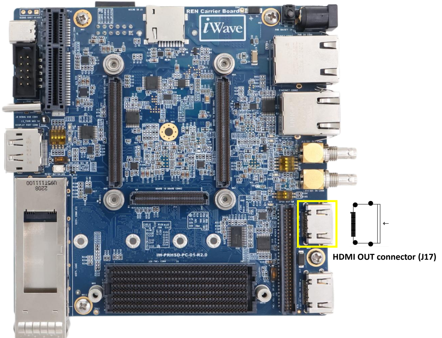
Figure 14: HDMI OUT Connector
