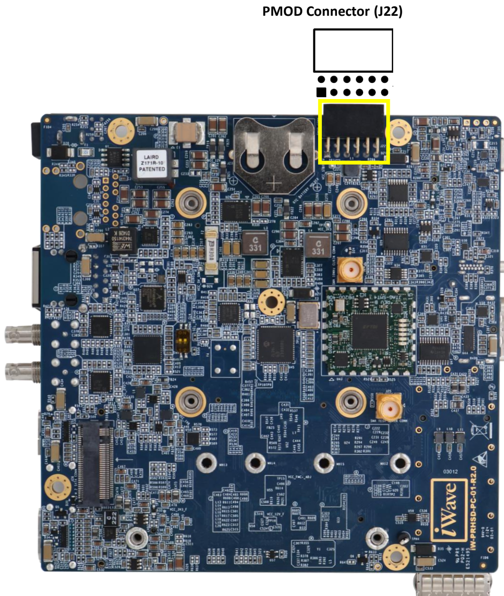
Figure 15: PMOD Host Connector
