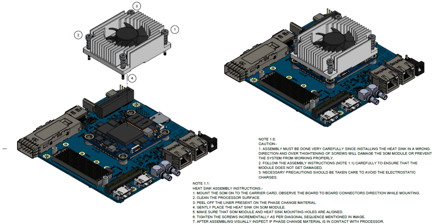
Figure 30: SOM with Fan sink fixing procedure
