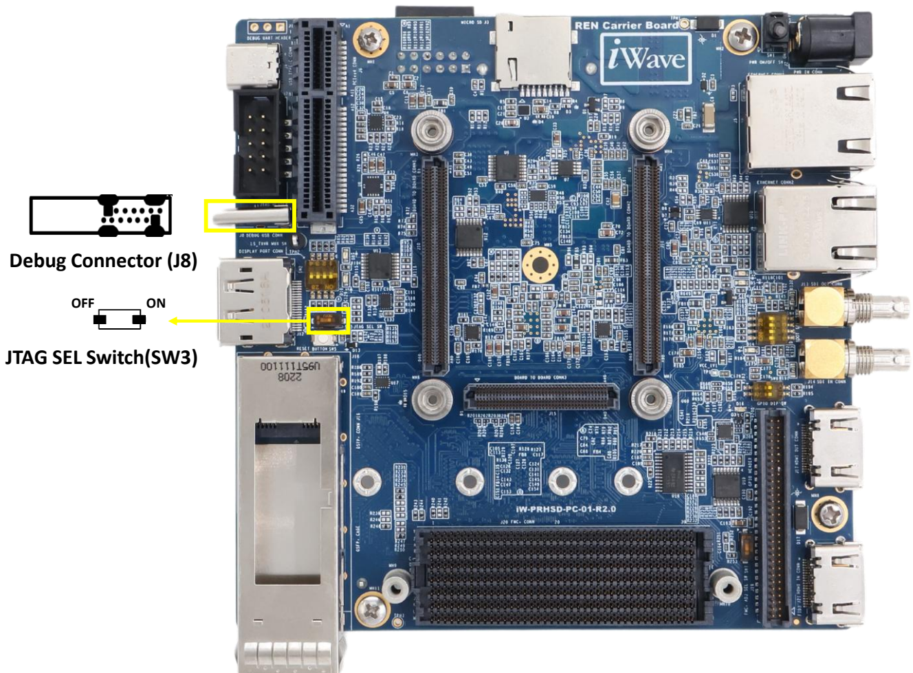
Figure 9: Debug Connector
