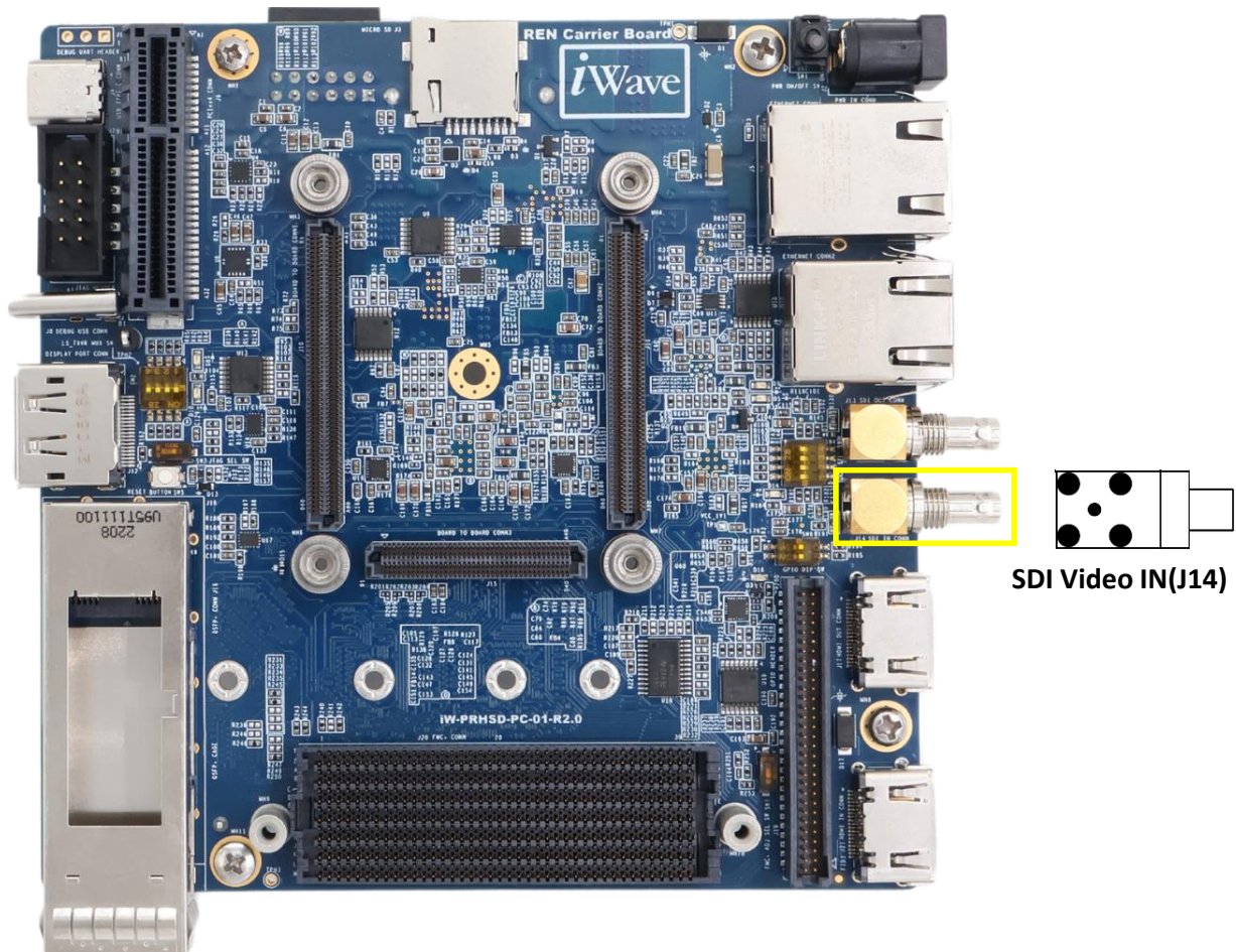
Figure 11: SDI Video IN
