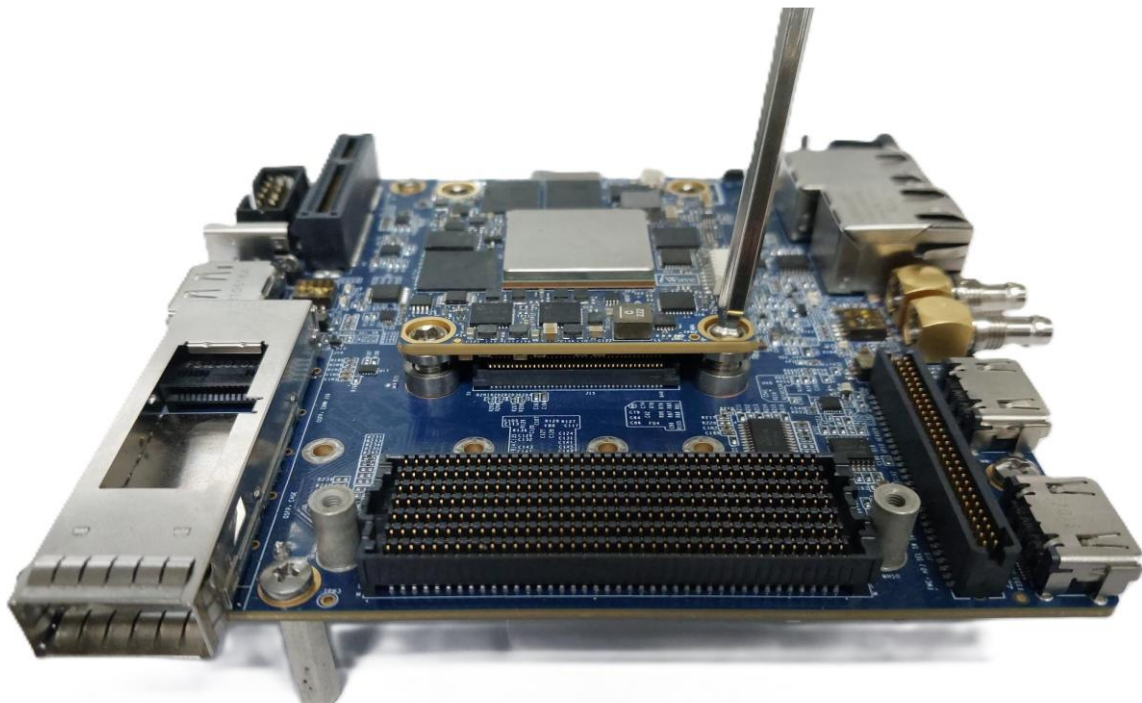
Figure 29: Removal SOM from Carrier Board
