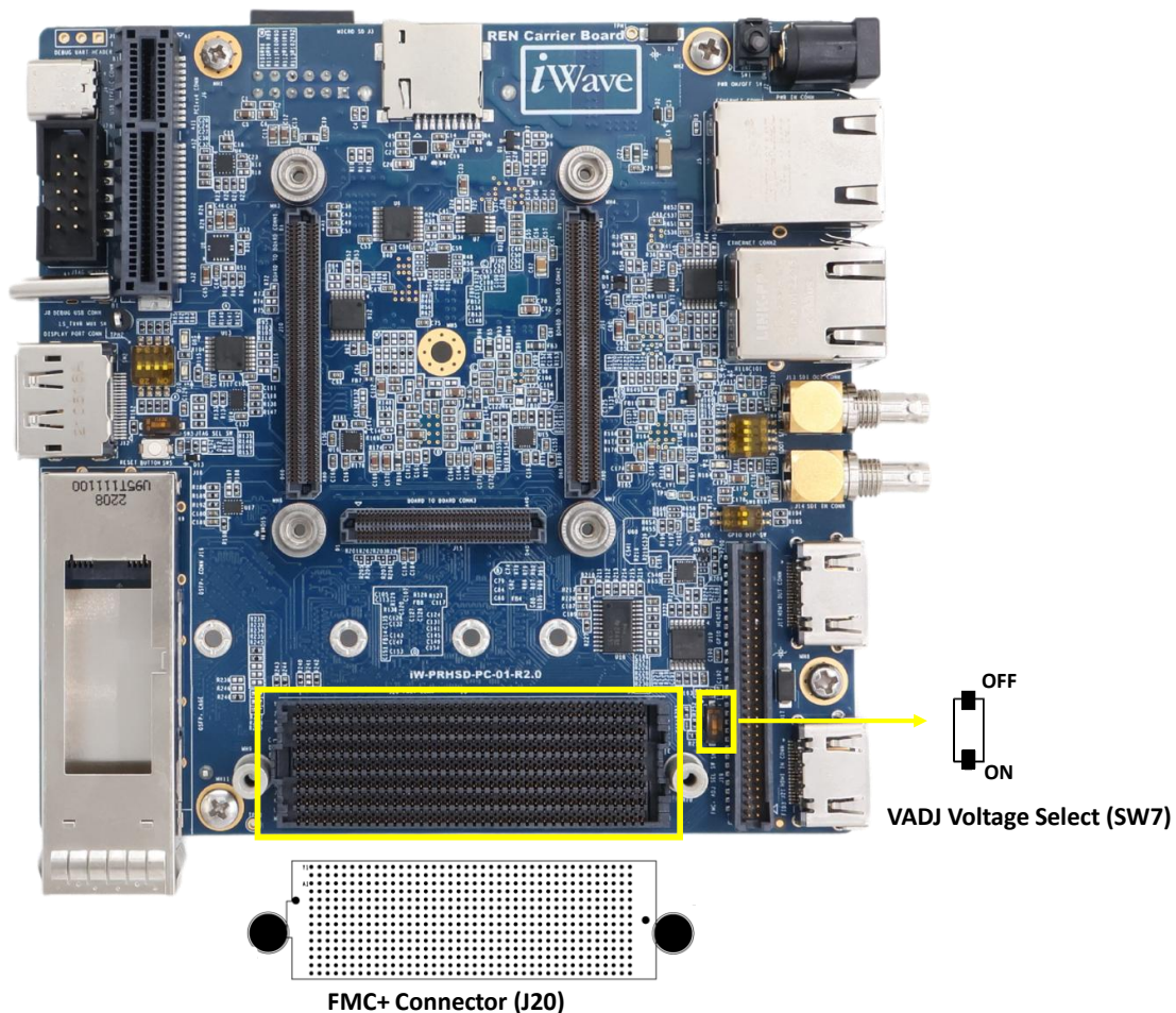
Figure 16: FMC+ Connector
