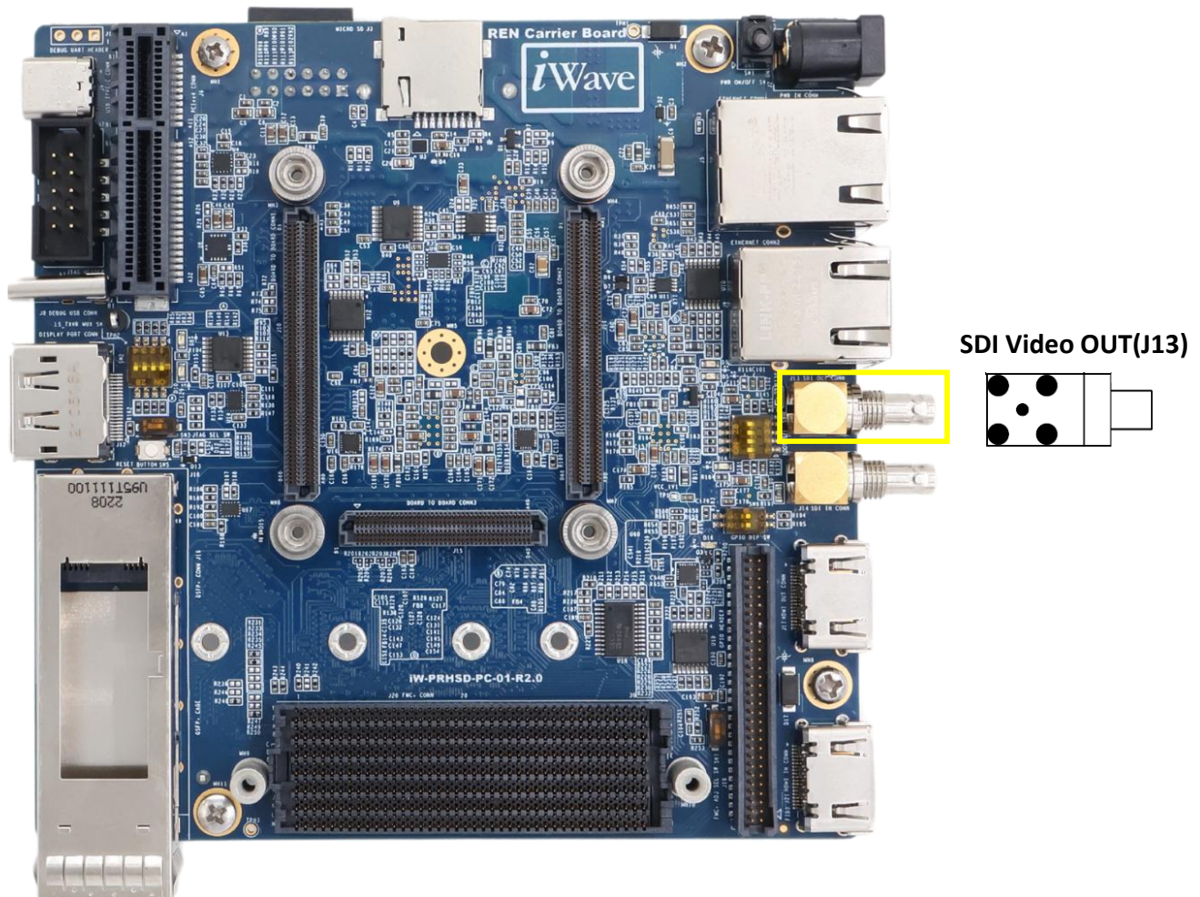
Figure 12: SDI Video OUT
