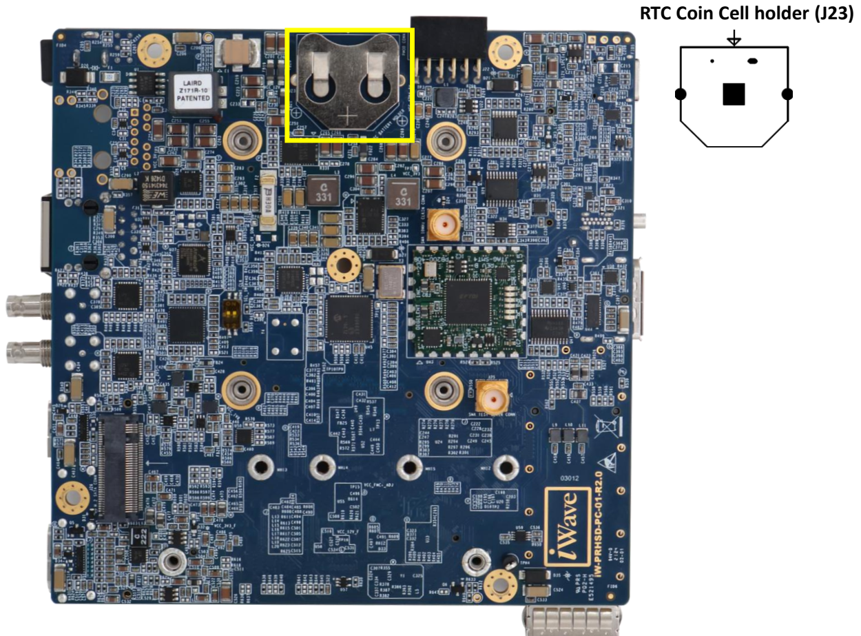
Figure 22: RTC Coin Cell Holder
