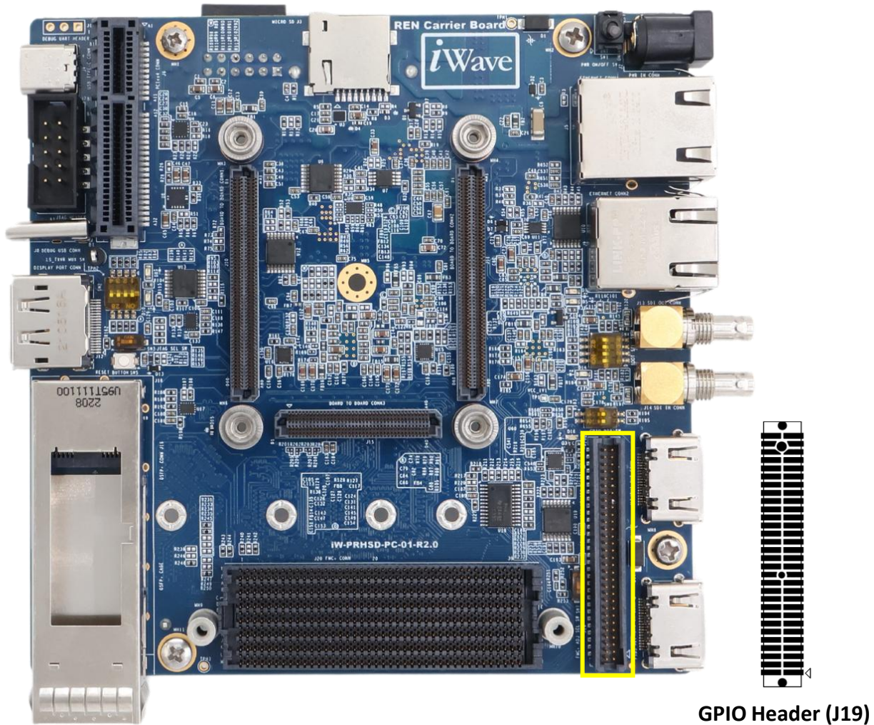
Figure 8: GPIO Header
