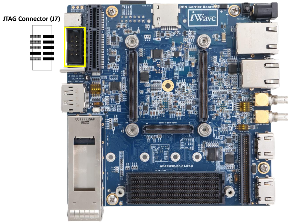
Figure 10: JTAG Connector
