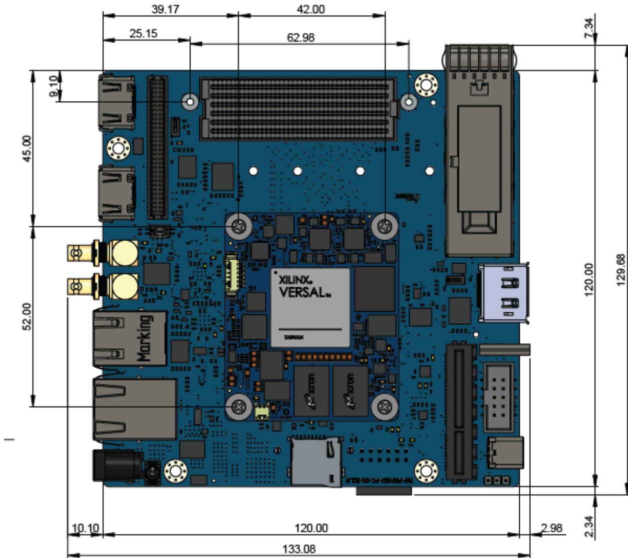
Figure 24: Carrier board Mechanical dimension – Top View
