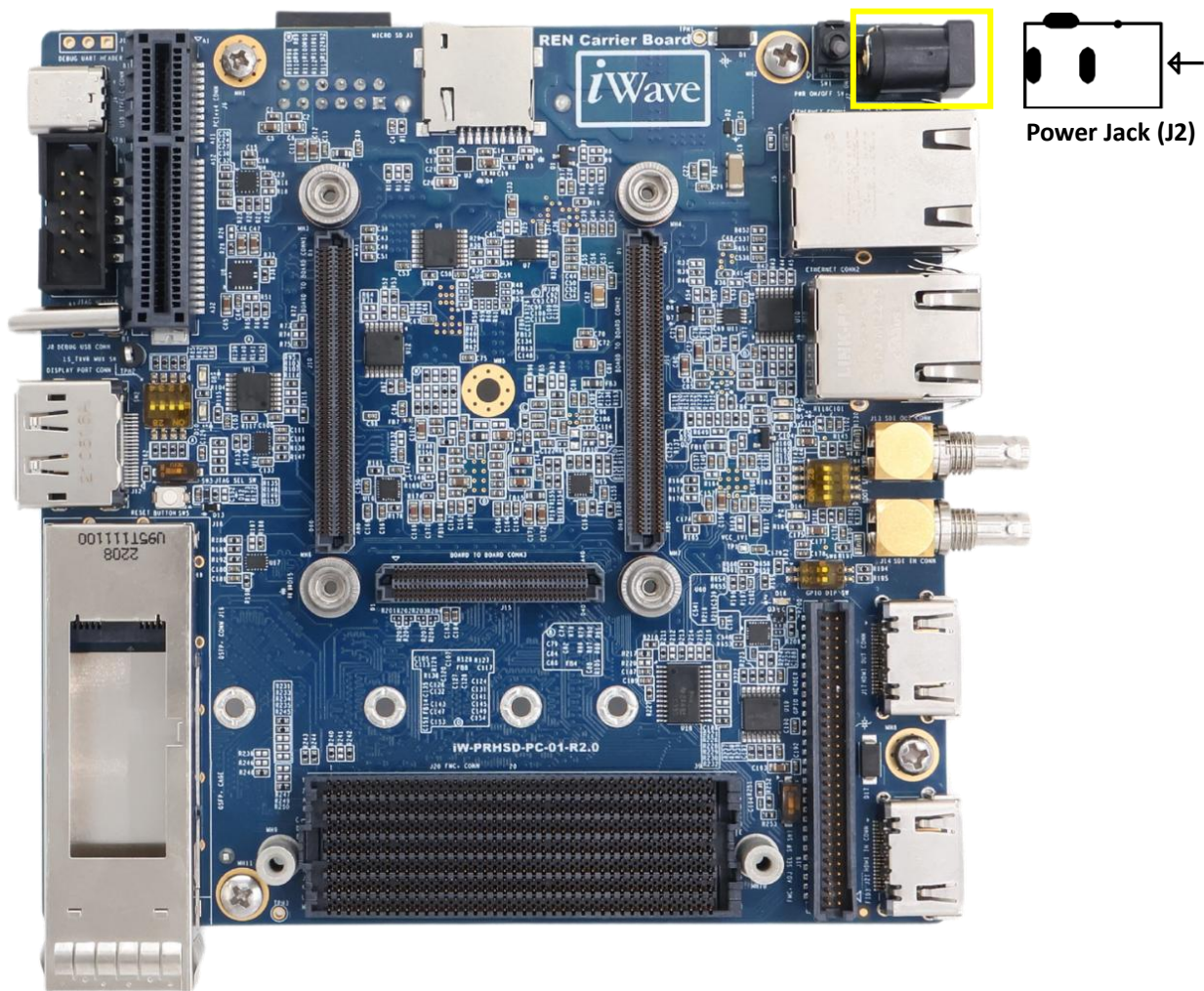
Figure 23: Power Jack
