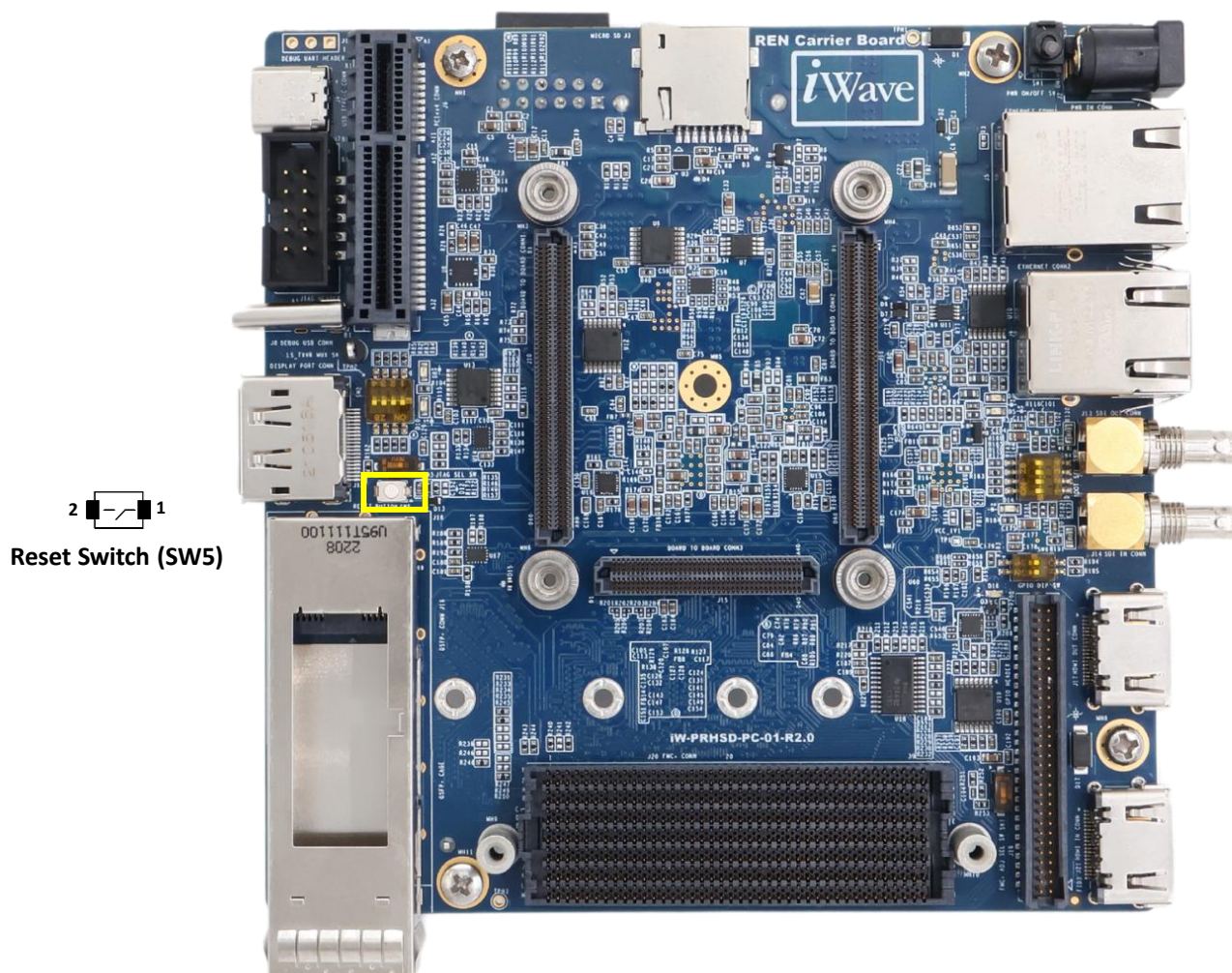
Figure 21: Reset Switch
