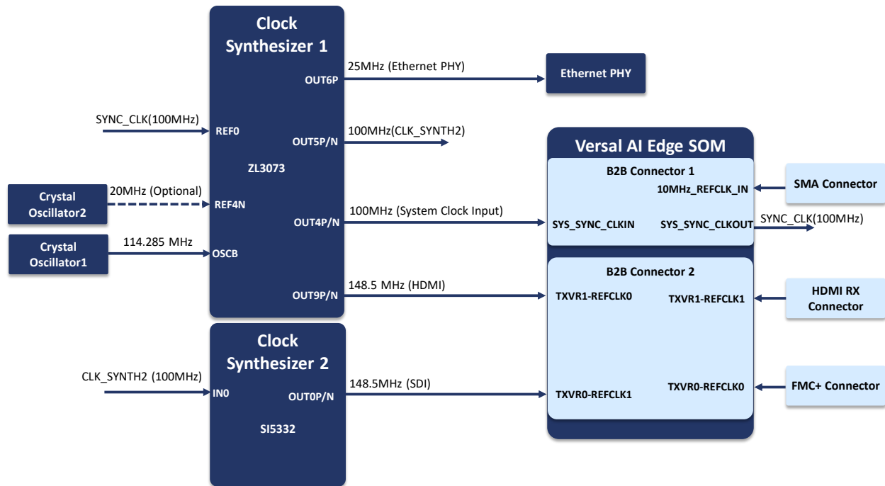
Figure 18: Clock Tree
