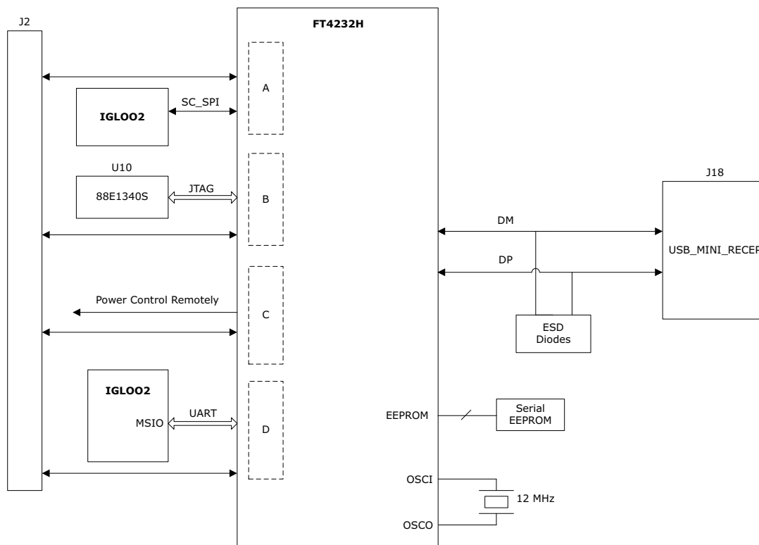
Figure 12 • FTDI Interface
