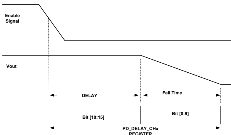
Fig. 21: Channel Soft-Stop Sequence
