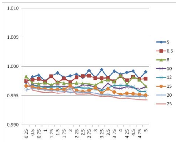
Fig. 20: Temperature and Voltage Regulation 1.0V OUT (±1% Vout window)
