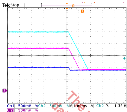
Fig. 16: CH1:1.0V CH2:5V CH3:1.8V Sequential Soft-Stop Configuration Vout Shutdown = 0.8V, No load
