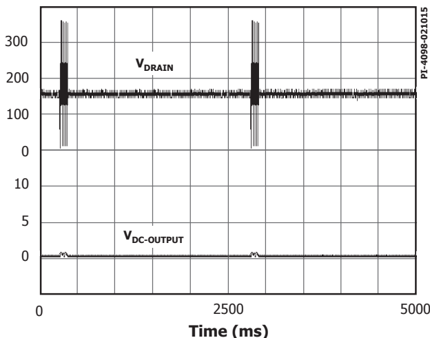
Figure 6. Auto-Restart Operation.
