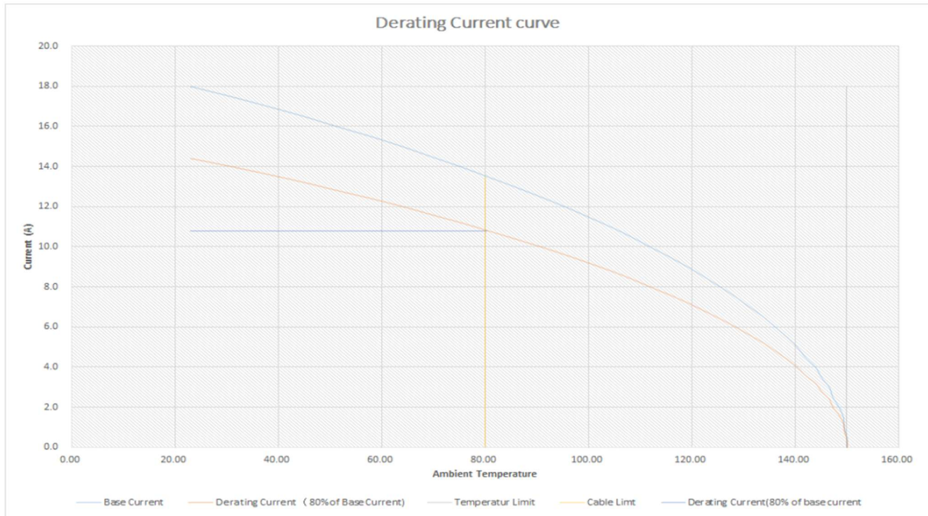
Figure 1: Derating curve 2-pin: 10.8A (angled/ straight)
