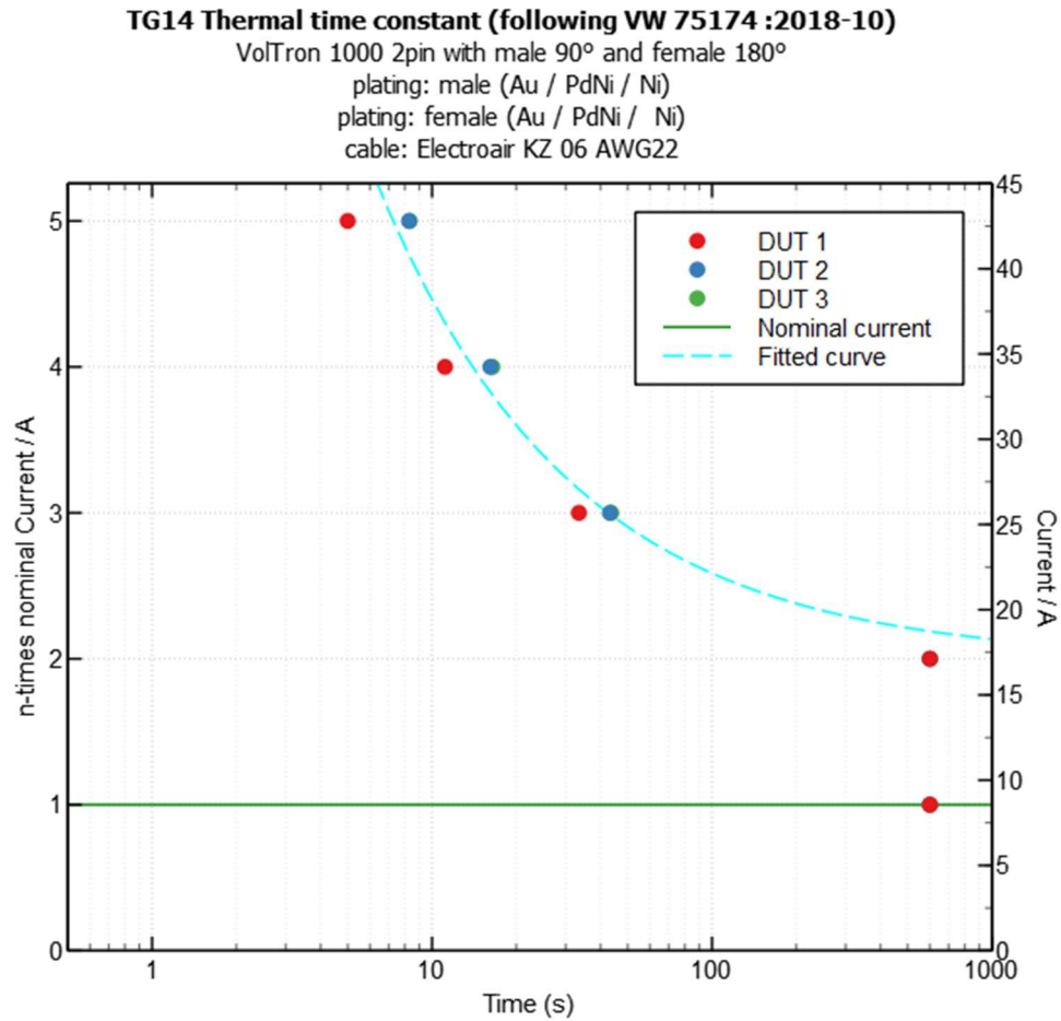
Figure 3: Thermal time constant: Current over time diagram
