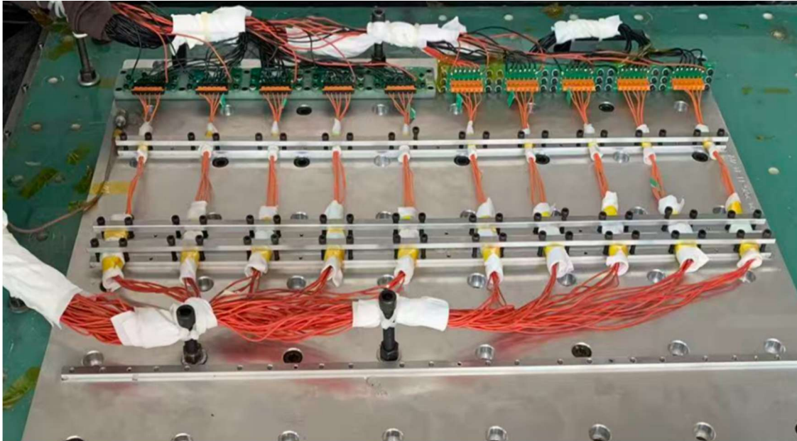
Figure 4: cable fastening distances of 100 mm and 250 mm
