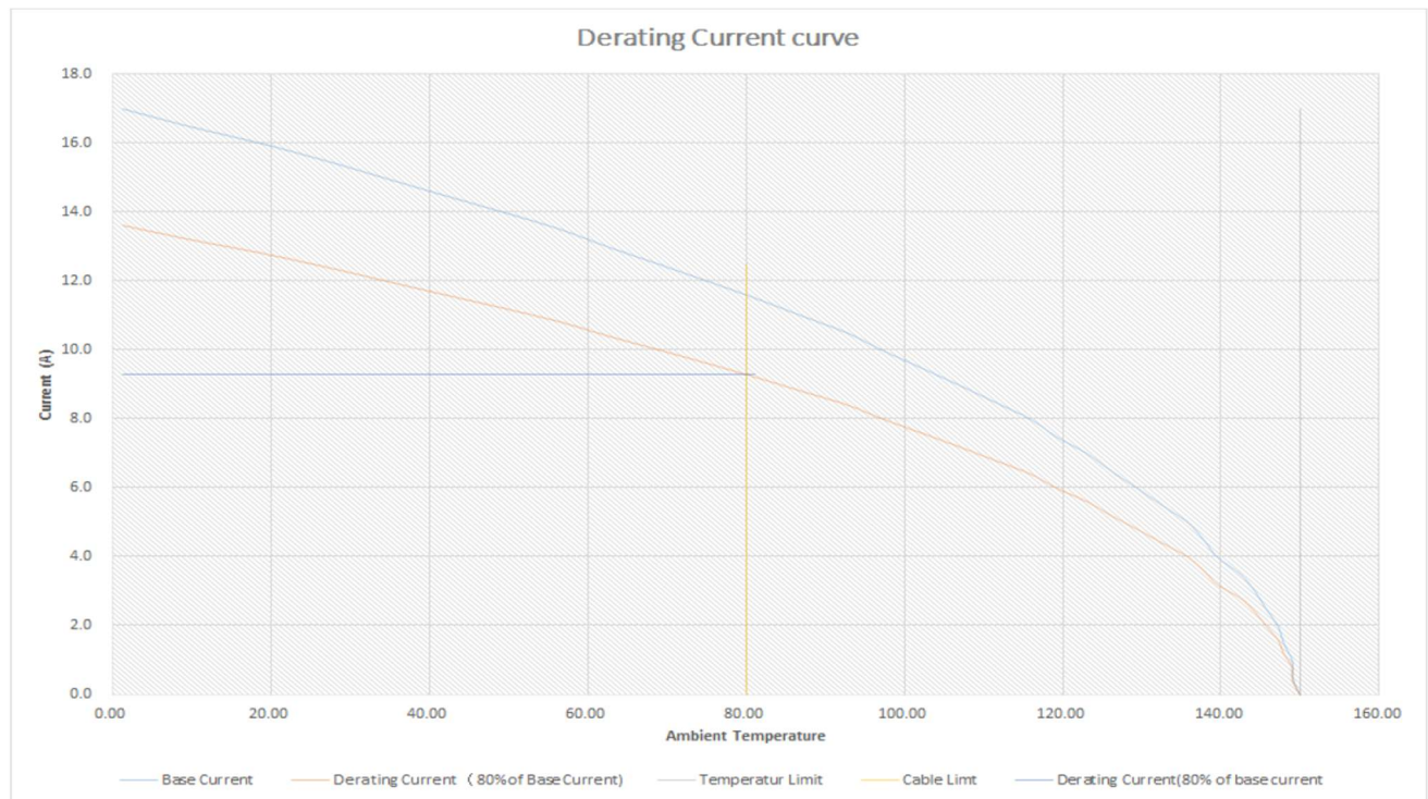
Figure 2: Derating curve 6-pin, 9.3A (angled/ straight)
