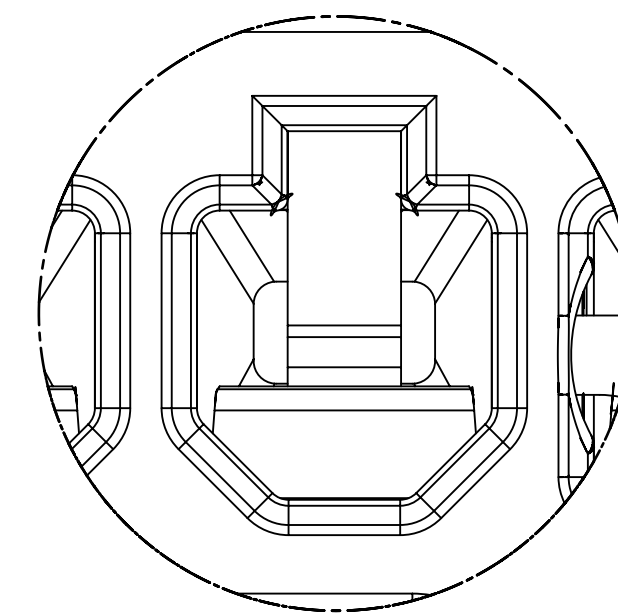
SHORTING BAR (SB) CIRCUITS ARE IDENTIFIED BY THE GROMMET CAP OPENING FEATURE SHOWN ABOVE. DETAIL 1 SCALE 15:1
