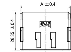
Guide Key: Common for Standard and Another Key Shape (2pos.)
