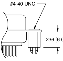
BL Option Bottom side riveted #4-40 Clinch Nuts with PCB Boardlocks
