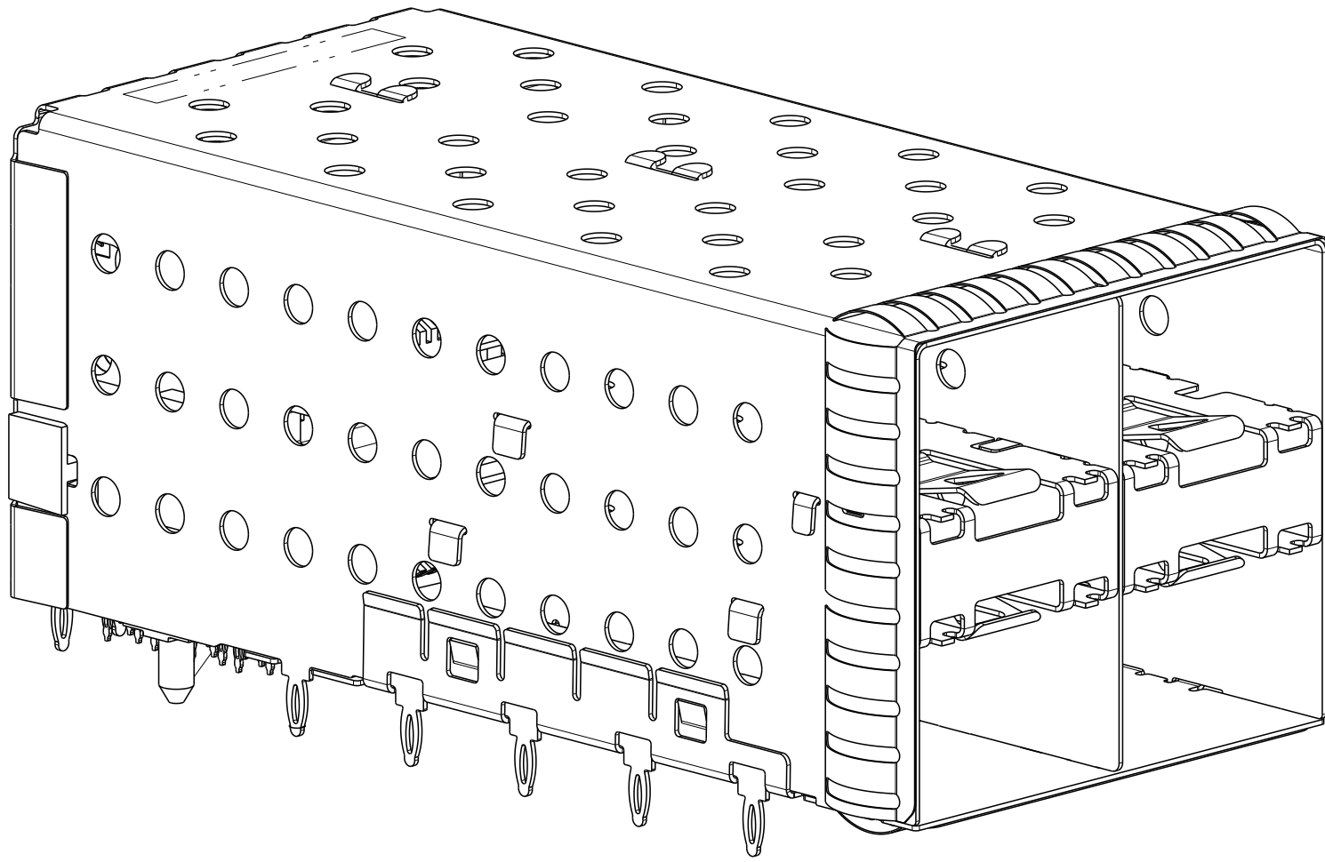
2007637-8 AND 1-2007637-8 SCALE 3:1
