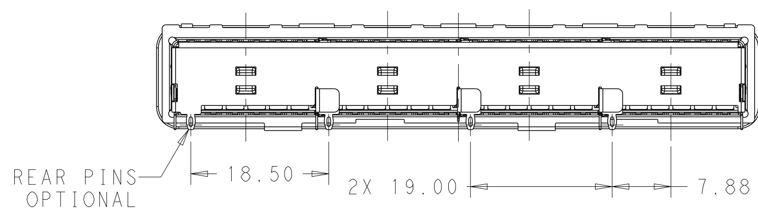
BACK VIEW SCALE 2:1
