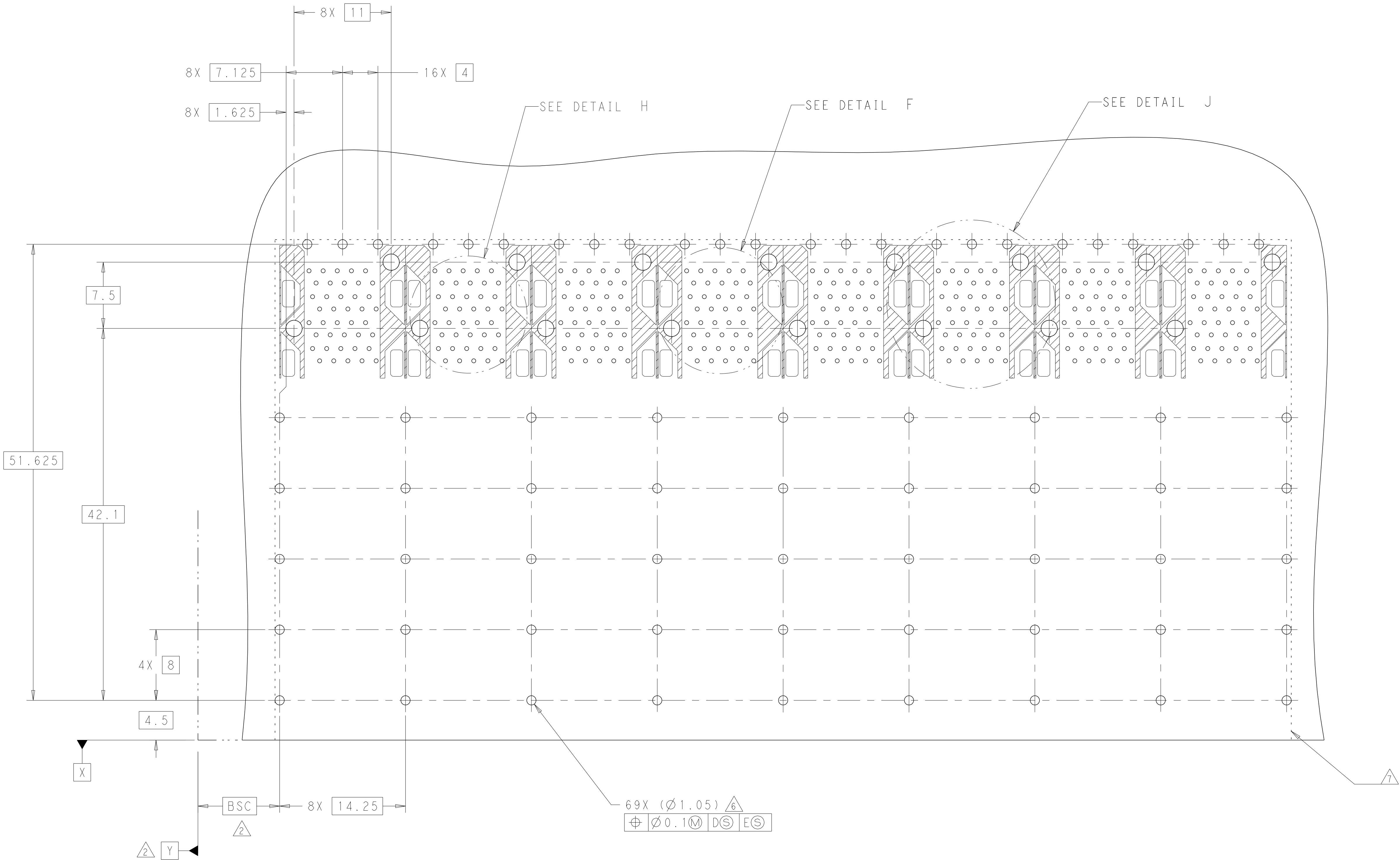
RECOMMENDED PCB LAYOUT COMPONENT SIDE OF BOARD SCALE 4:1
