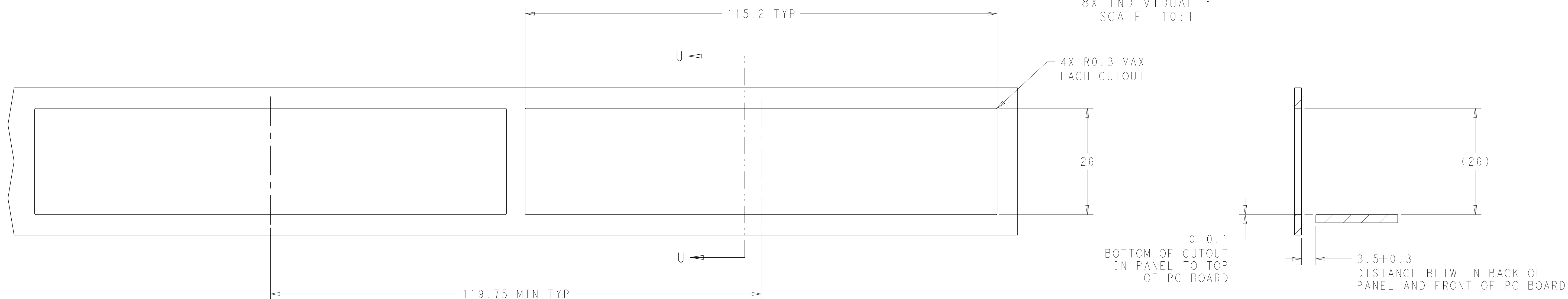
SECTION U-U SCALE 2:1
