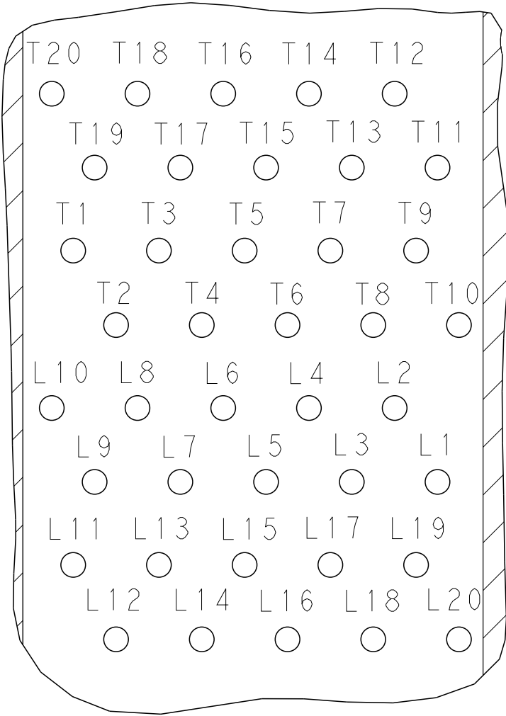
DETAIL H CONNECTOR PIN-OUT COMPONENT SIDE OF BOARD 8X INDIVIDUALLY SCALE 10:1
