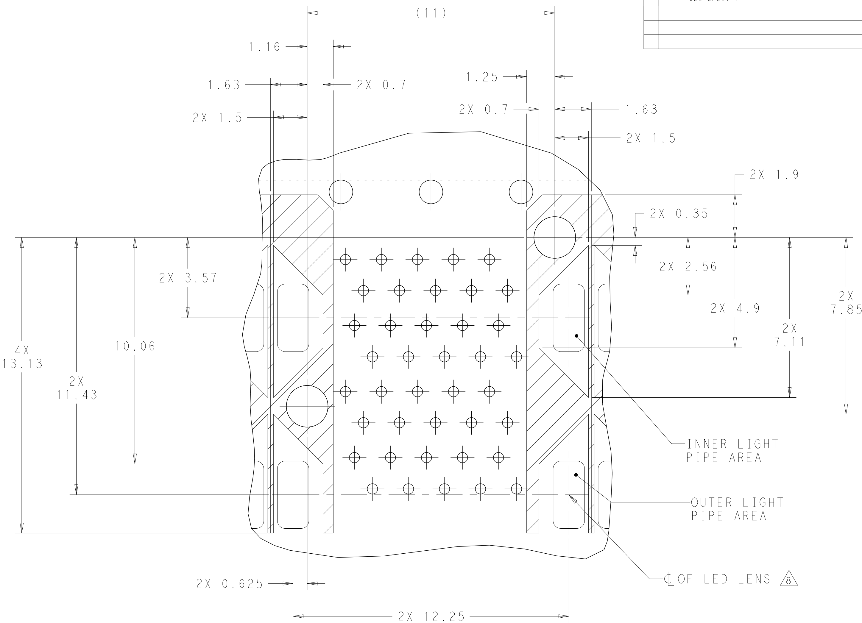
DETAIL J CONNECTOR HOUSING KEEPOUT ZONE 8X INDIVIDUALLY SCALE 10:1
