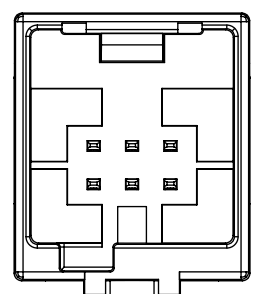
6 CIRCUIT
