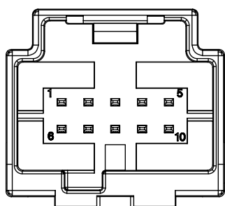
10 CIRCUIT
