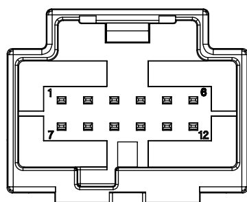
12 CIRCUIT
