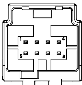
8 CIRCUIT
