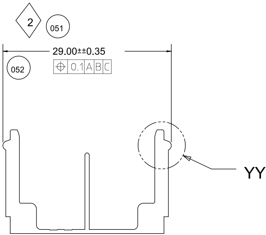
SECTION F-F (RELEASE FEATURE)
