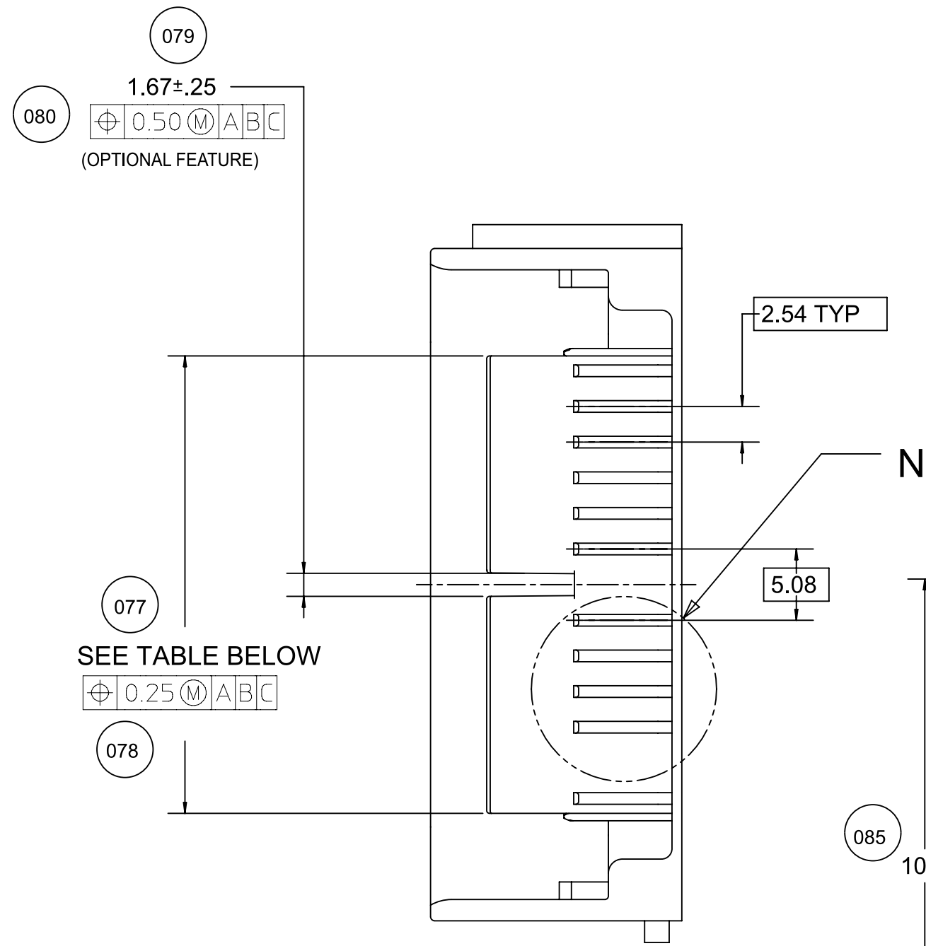
SECTION J-J
