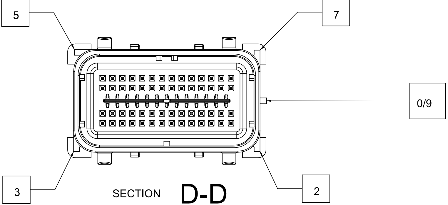
SECTION D-D 56 CKT COMPONENT CONNECTOR INTERFACE KEY OPTION K SHOWN
