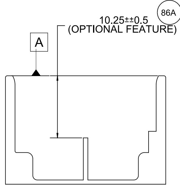
SECTION J-J
