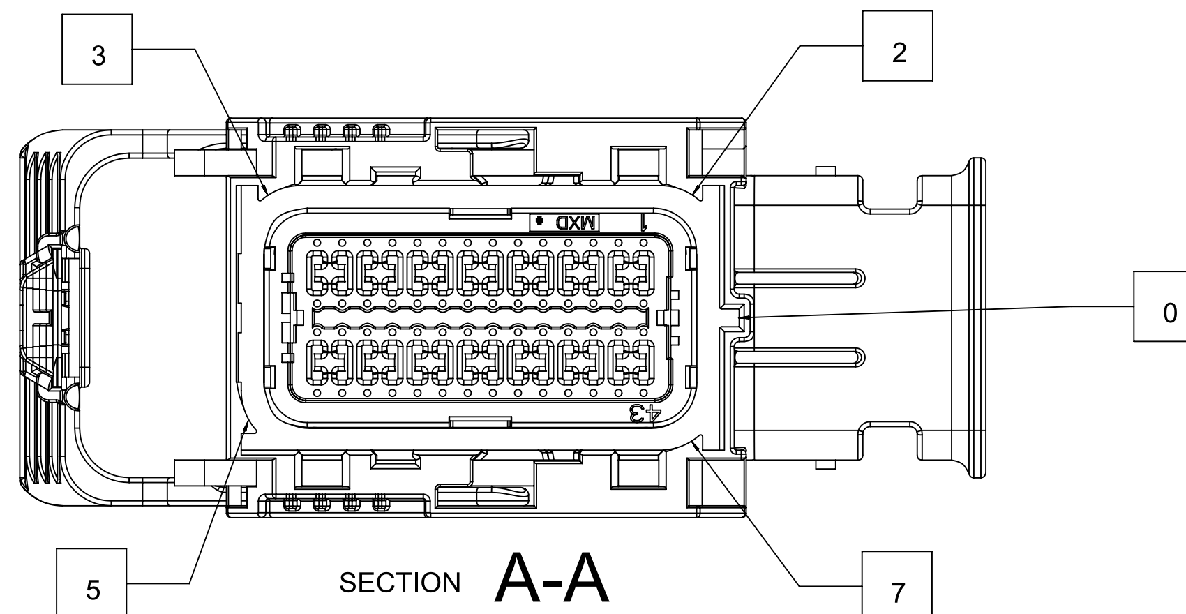
56 CKT HARNESS CONNECTOR ASSEMBLY KEY OPTION K SHOWN
