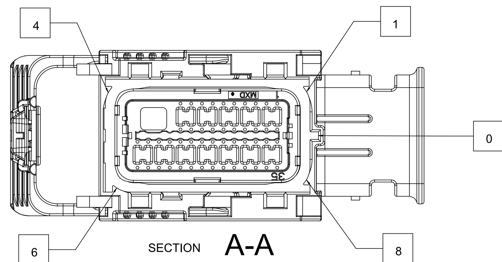
49 CKT HARNESS CONNECTOR ASSEMBLY KEY OPTION B SHOWN
