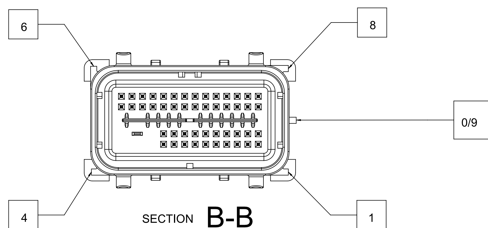
49 CKT HARNESS CONNECTOR ASSEMBLY KEY OPTION B SHOWN
