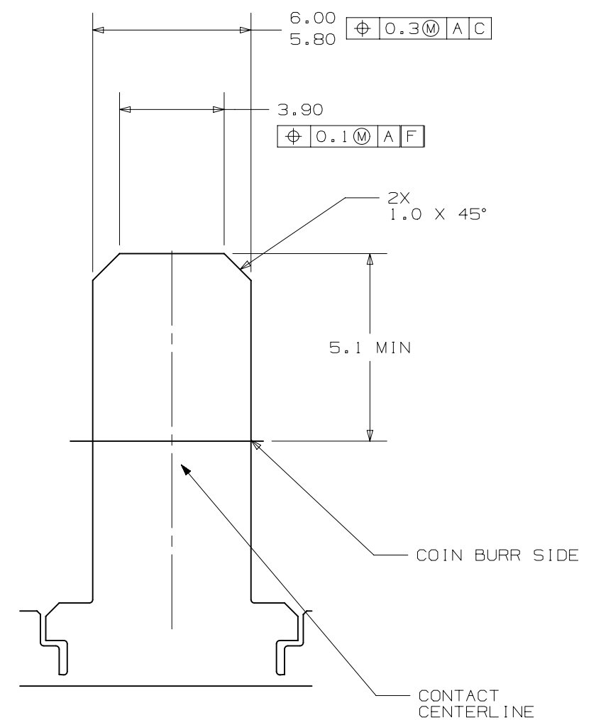
SECTION CB-CB
