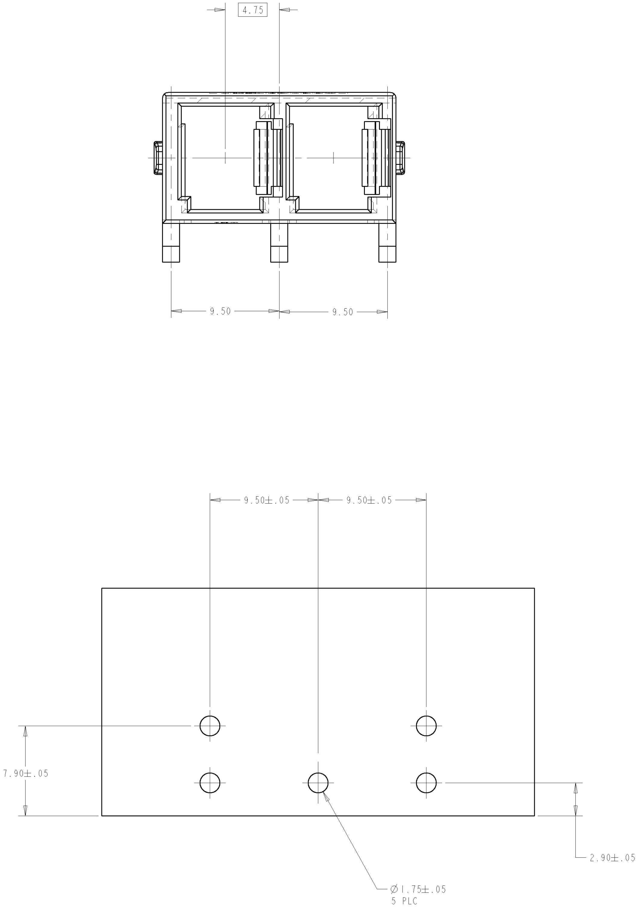
RECOMMENDED HOLE PATTERN SCALE 5:1
