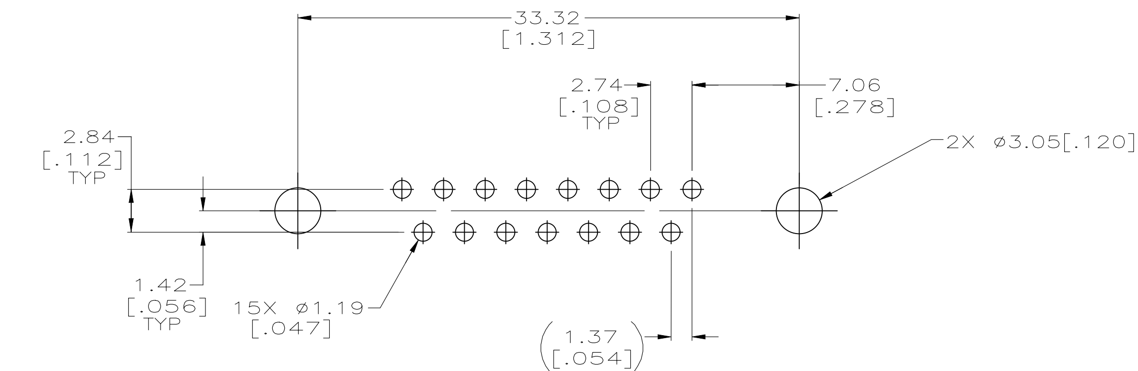
RECOMMENDED PC BOARD MOUNTING DIMENSIONS
