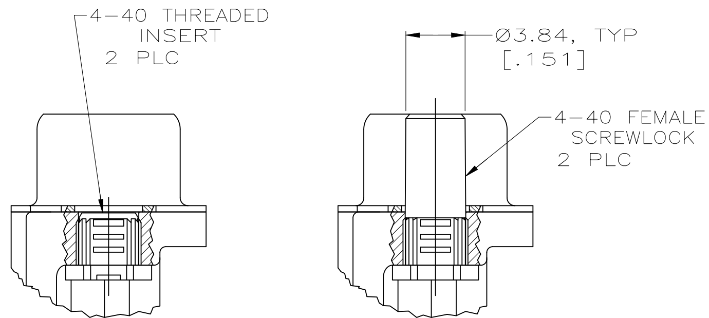
DETAIL D
