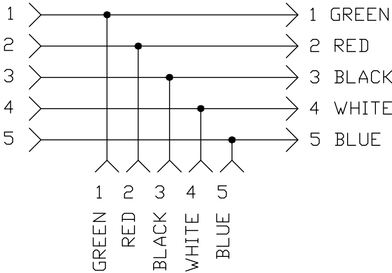
ELECTRICAL DIAGRAM
