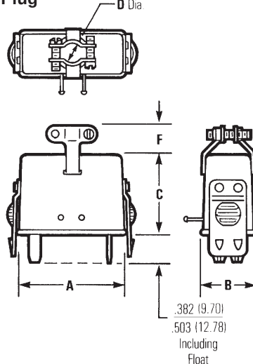
Plug
