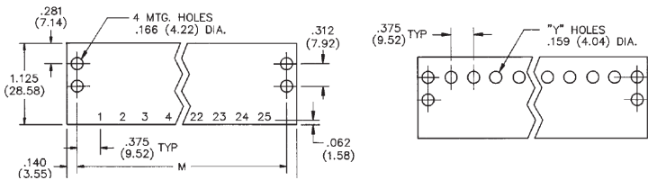
"Y" Terminal
