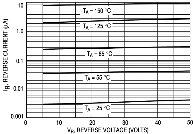
Figure 2. Leakage Current
