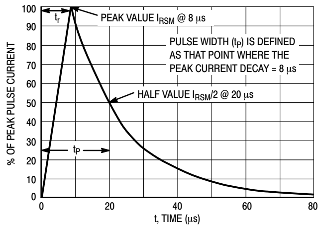
Figure 2. Pulse Waveform 8 \times 20\text{ }\mu\text{s}
