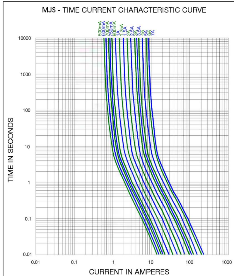
Average Time Current Curve
