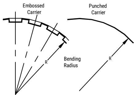
Figure 4 – Bending Radius
