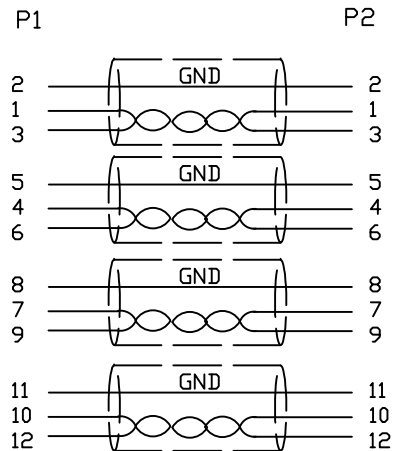
1.Wiring Diagram.
