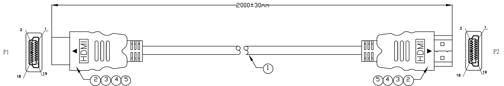
1.Wiring Diagram.
