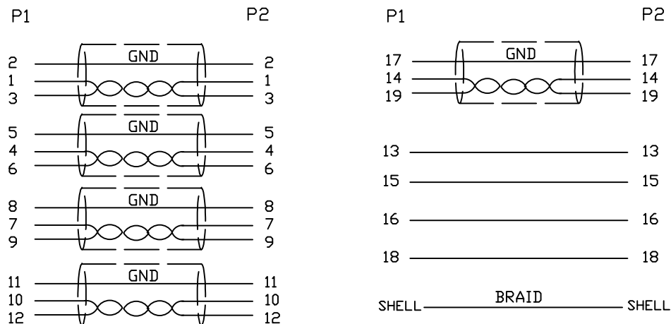
1.Wiring Diagram.
