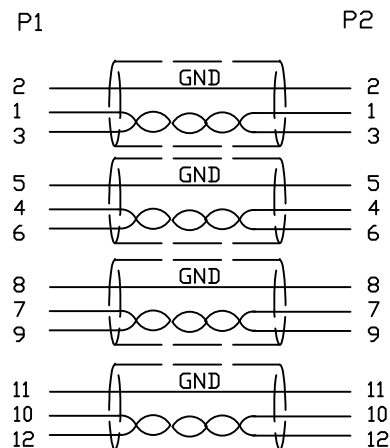
1.Wiring Diagram.
