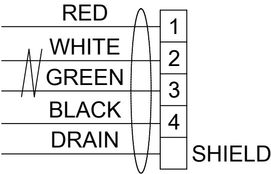
WIRE DIAGRAM
