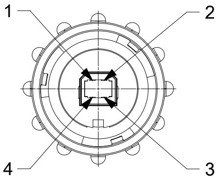
USB-TYPE B MALE FACE VIEW
