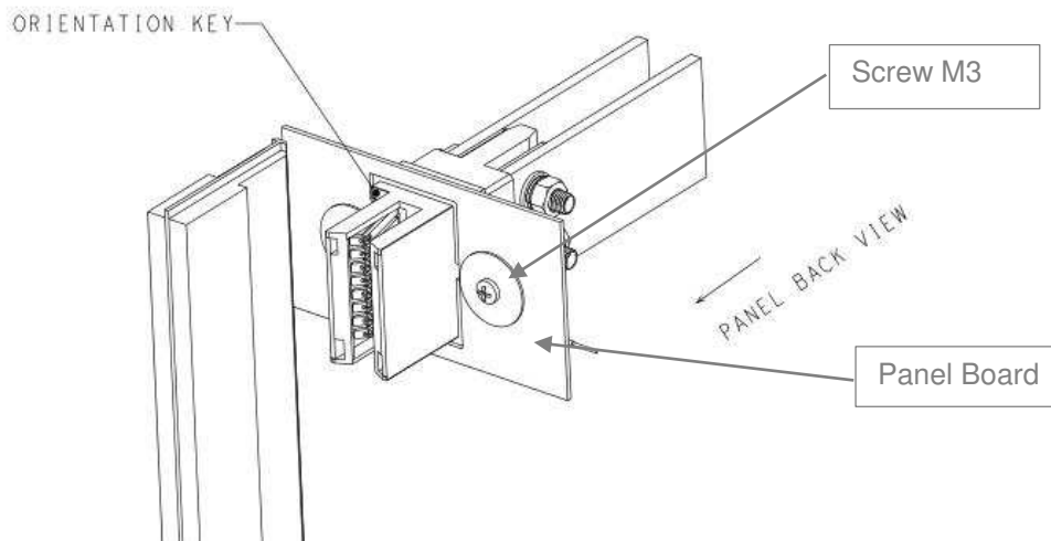
Figure 3. The reference panel board assembly view
