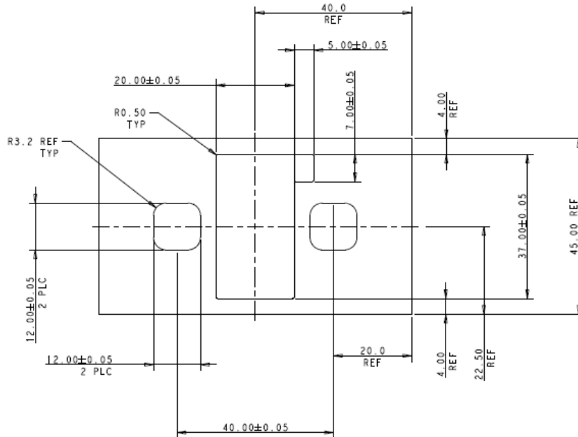
Figure 2 The recommended panel board layout view for Dual-Pole 500A Rack Bus Bar Power Connector.
