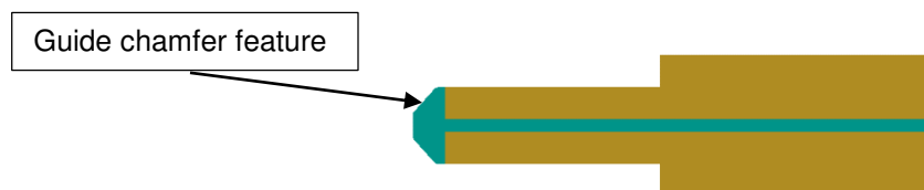
Figure 4. Recommended guide chamfer feature(2.0*2.0mm) view of Laminated Mating Bus Bar Board.
