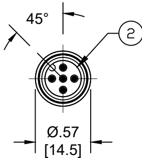
MALE INSERT- FACE VIEW
