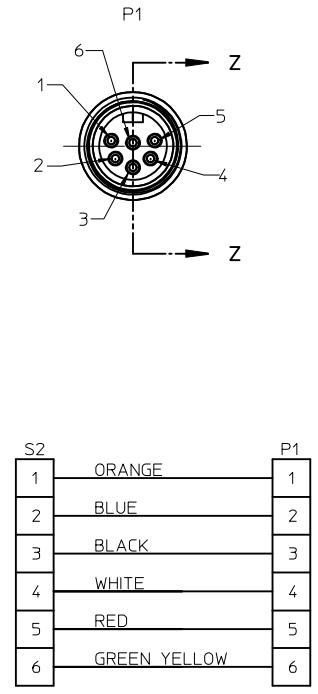
WIRING DIAGRAM
