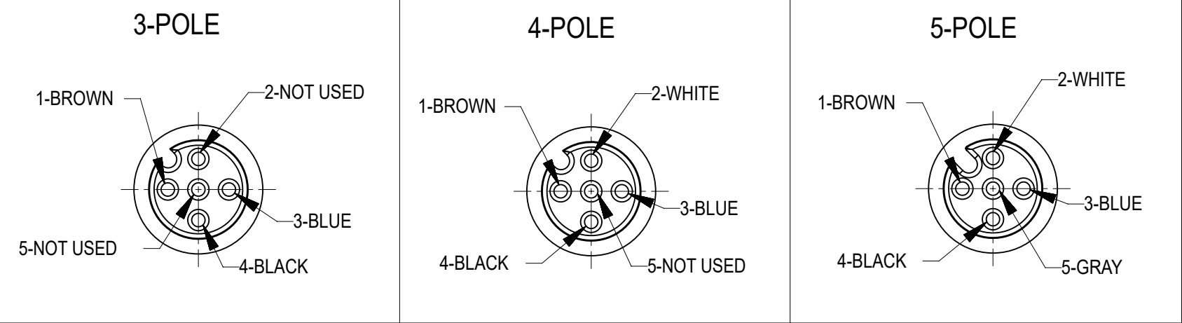
FRONT VIEW - FEMALE INSERT CONFIGURATION CHART
