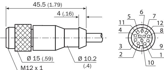
Dimensions in mm (inch)
