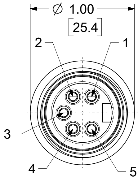
MALE FACE VIEW
