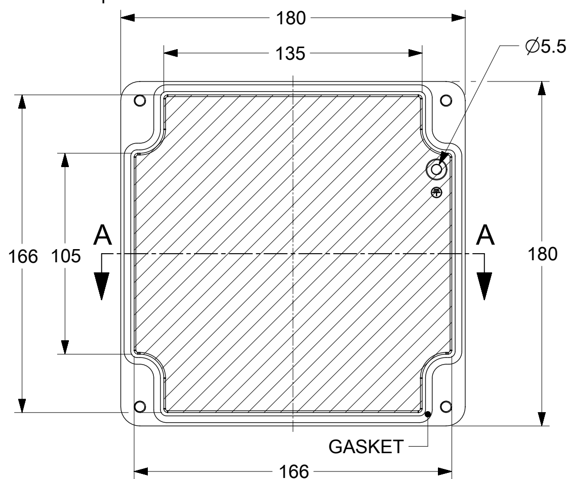
Cover/Coperchio
