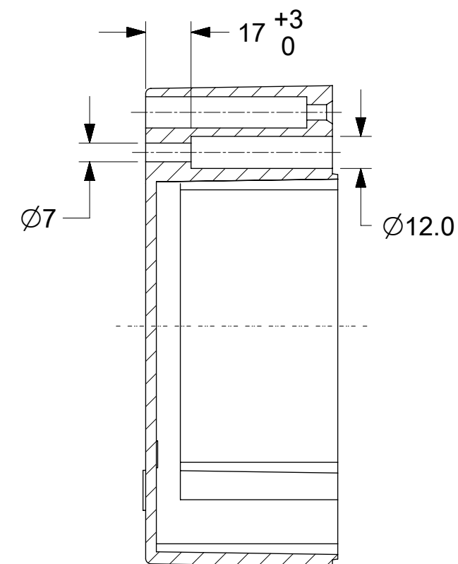
SECTION C-C
