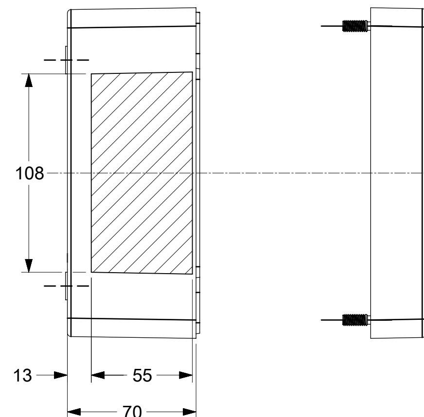
Side/Lato A
