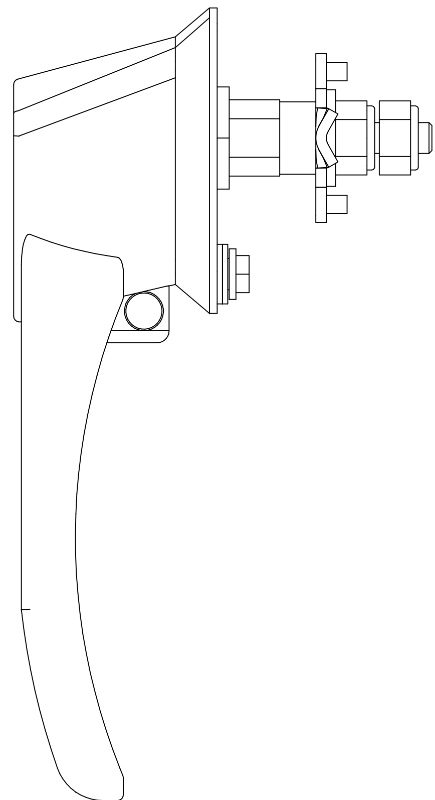
SIDE VIEW
