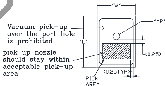
Recommended Vacuum Nozzle Pickup Top View
