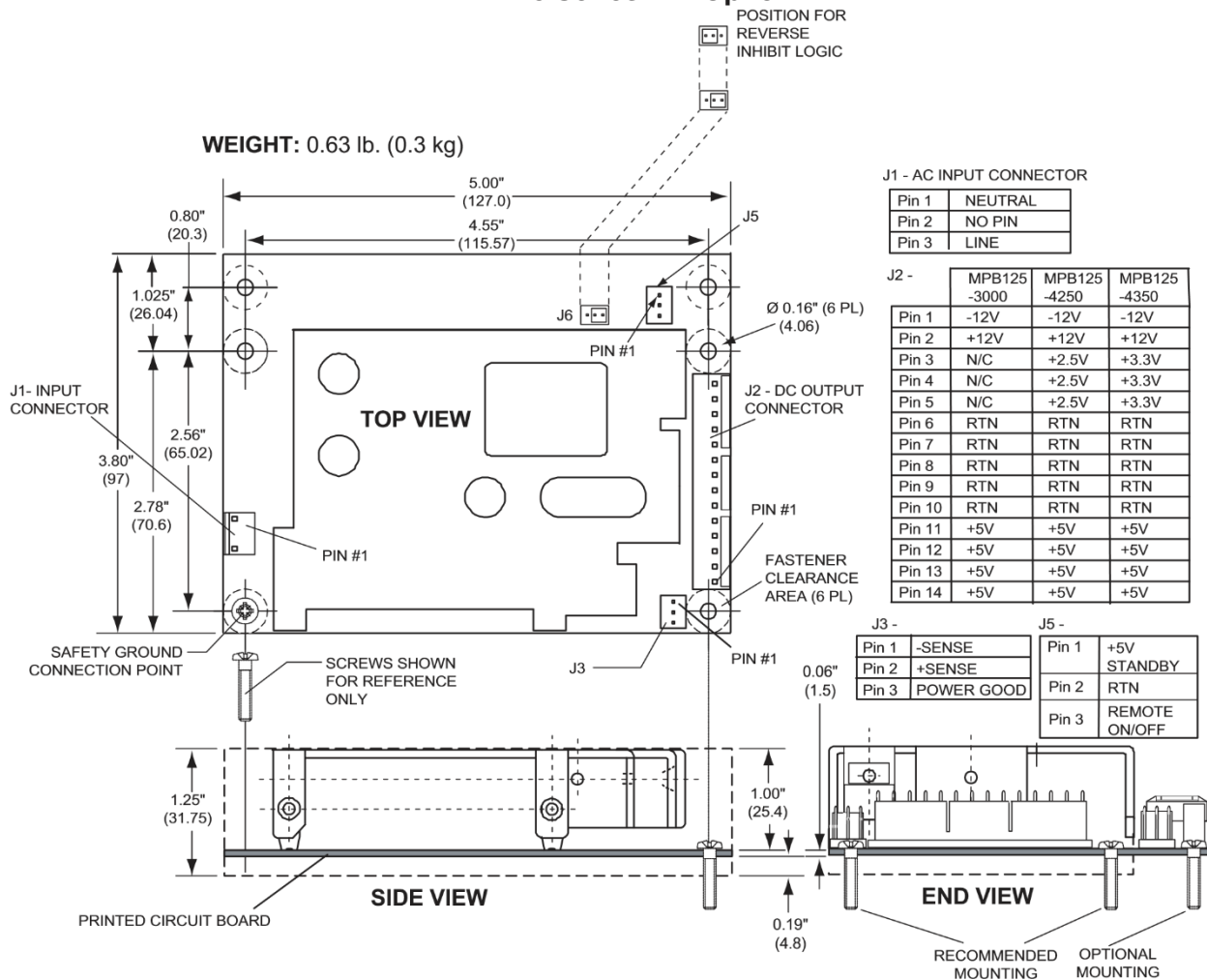
Mechanical Drawing (-3000R, -4250R, &amp; -4350R Models)
