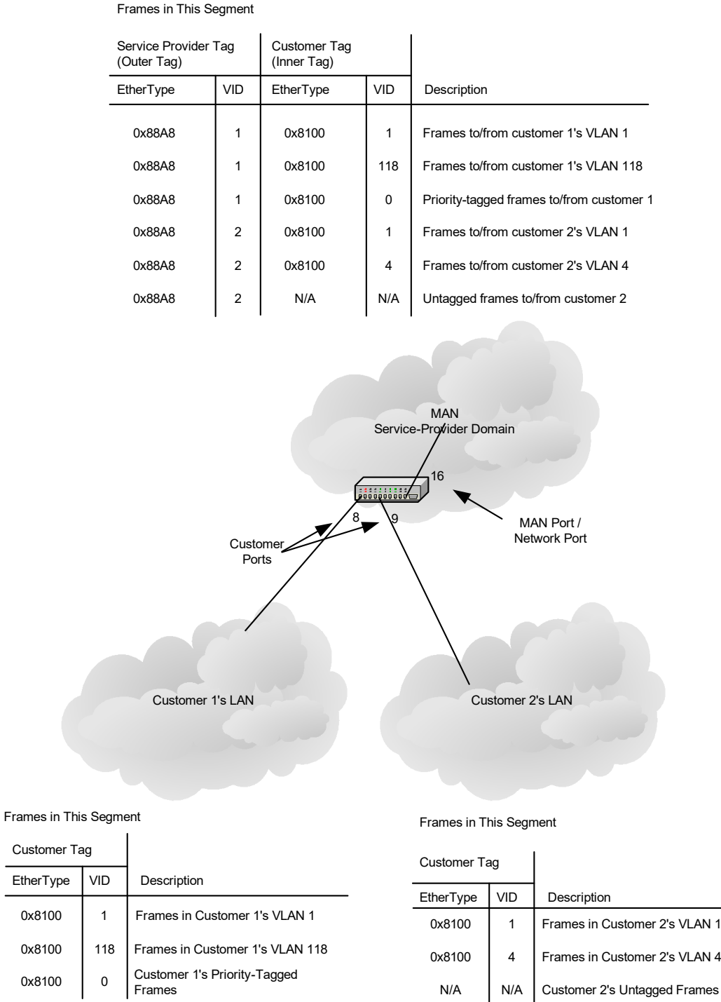
FIGURE 4-1: MAN ACCESS SWITCH SETUP
