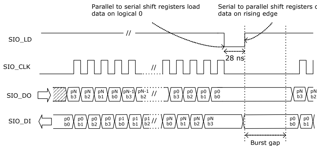
FIGURE 3-13: SIO TIMING
