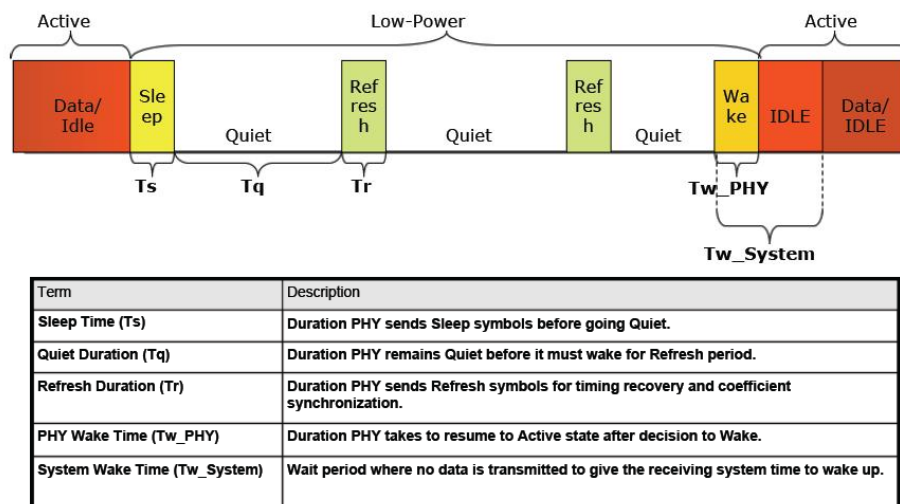
FIGURE 2-4: ENERGY EFFICIENT ETHERNET
