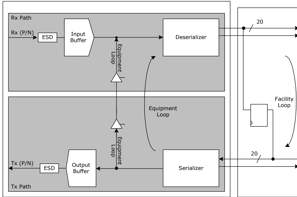
FIGURE 2-1: SERDES LOOPBACK
