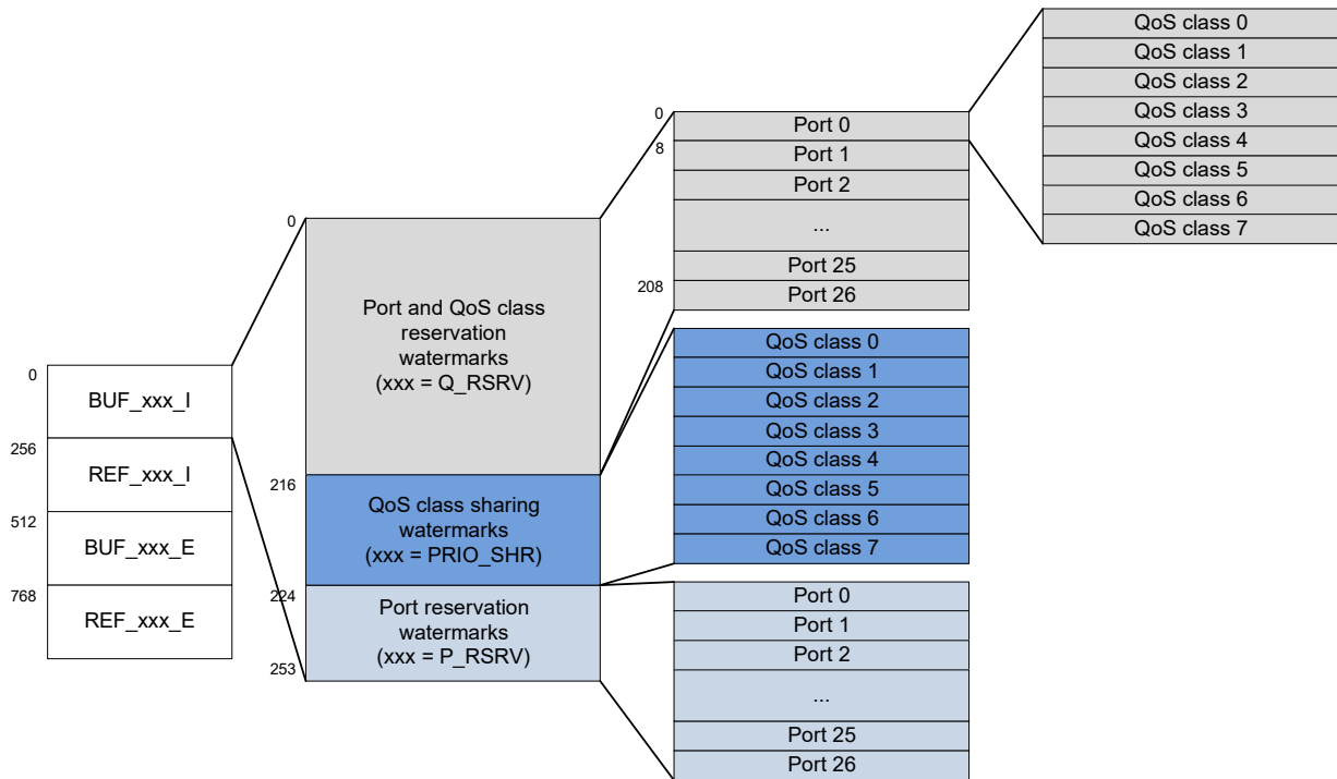
FIGURE 2-18: WATERMARK LAYOUT
