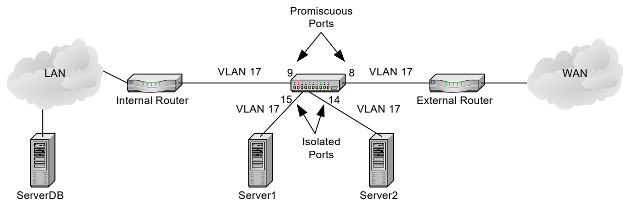
FIGURE 4-3: DMZ EXAMPLE FOR PRIVATE VLAN
