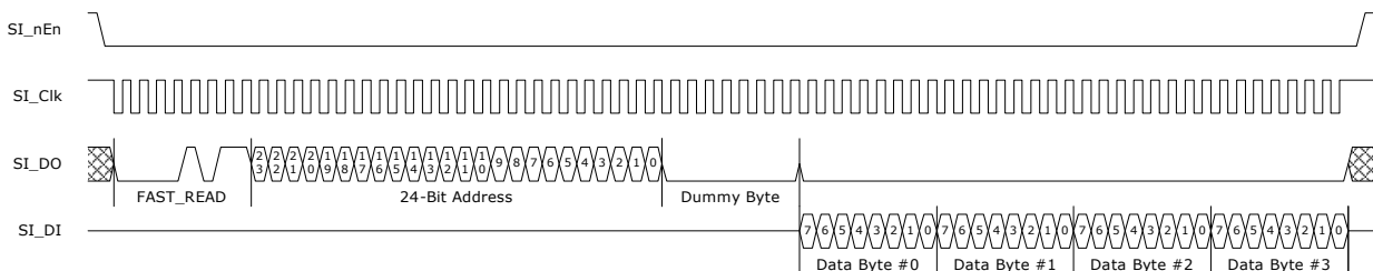
FIGURE 3-4: SI READ TIMING IN FAST MODE
