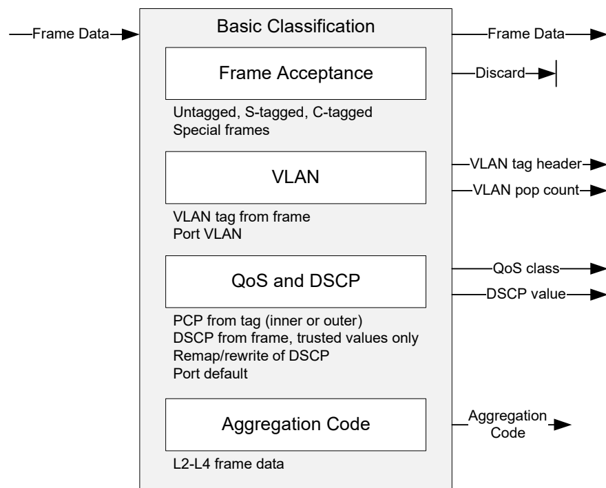
FIGURE 1-2: FRAME CLASSIFICATION
