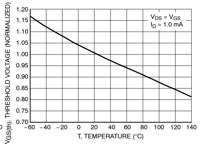
Figure 9. Temperature versus Gate Threshold Voltage
