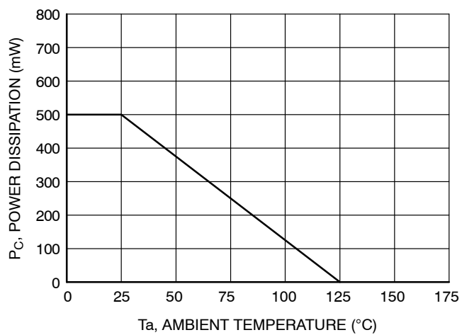
Figure 7. Power Derating
