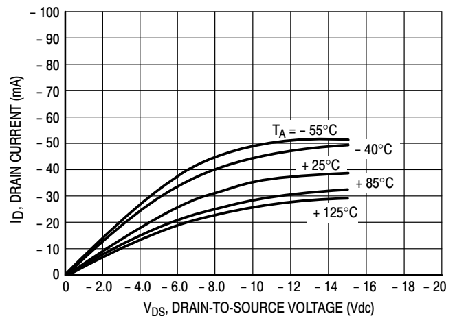
Figure 7. V_{GS} = -15 Vdc
