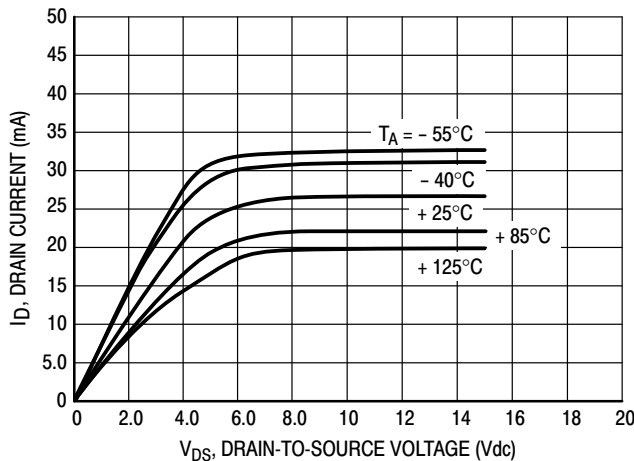
Figure 6. V_{GS} = 15 Vdc
