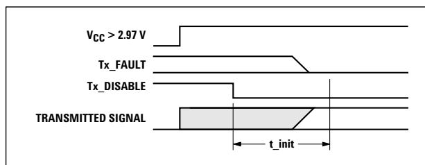
t_{\text{init}} : TX DISABLE ASSERTED
