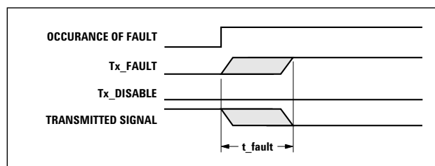
t_{\text{fault}} : TX FAULT ASSERTED, TX SIGNAL NOT RECOVERED
