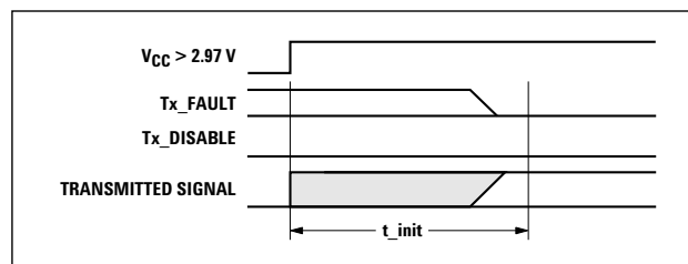
t_{\text{init}} : TX DISABLE NEGATED
