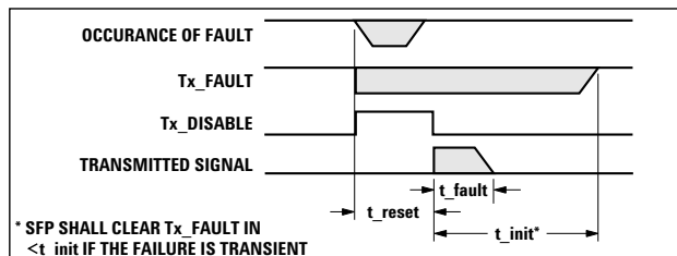
t_{\text{fault}} : TX DISABLE ASSERTED THEN NEGATED, TX SIGNAL NOT RECOVERED
