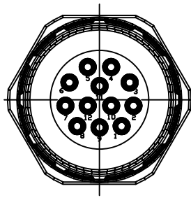
12-Pole
