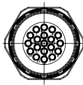
19-Pole (16+3)
